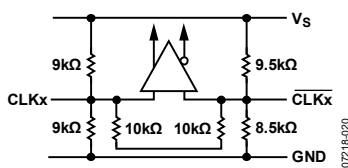
Figure 20. ADCLK854 Input Stage
