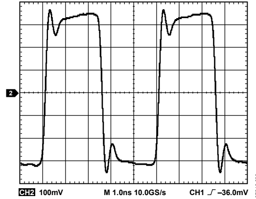
Figure 6. LVDS Output Waveform @ 200 MHz
