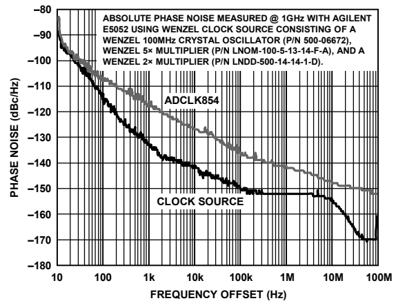
Figure 12. Absolute Phase Noise LVDS @ 1000 MHz
