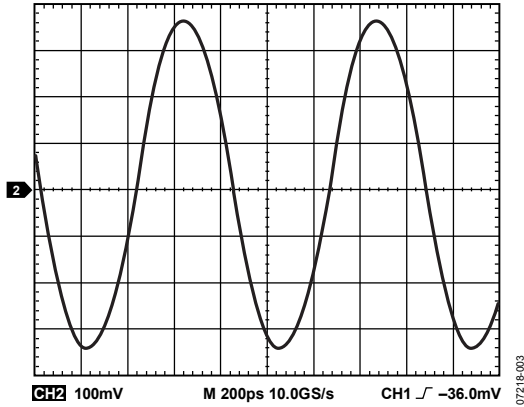
Figure 3. LVDS Output Waveform @ 1200 MHz
