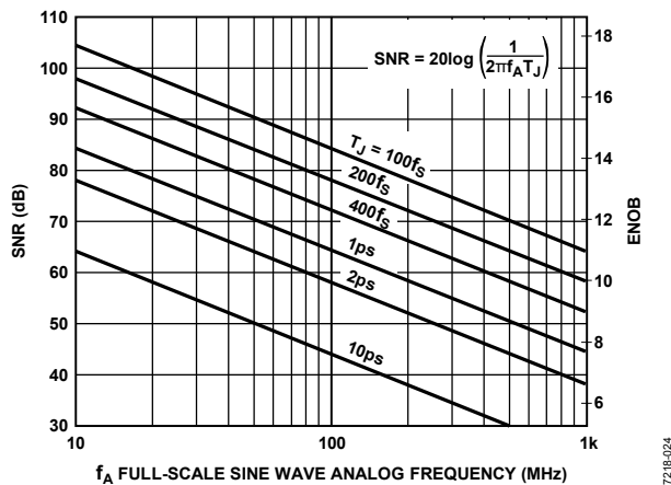
Figure 24. SNR and ENOB vs. Analog Input Frequency
