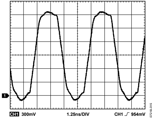
Figure 15. CMOS Output Waveform @ 200 MHz (10 pF Load)
