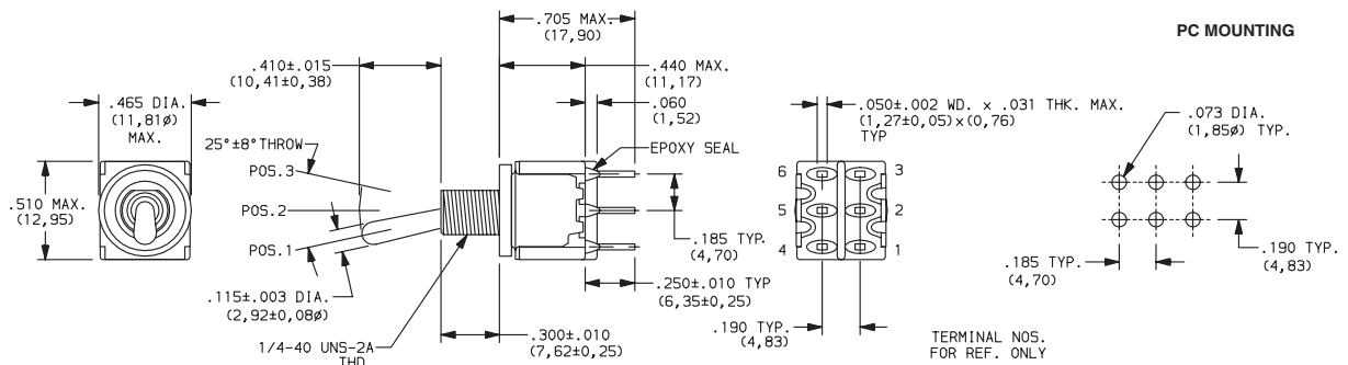
DPDT
