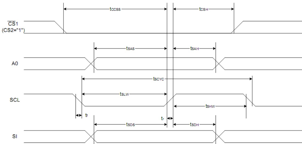
The 4-line SPI Interface
