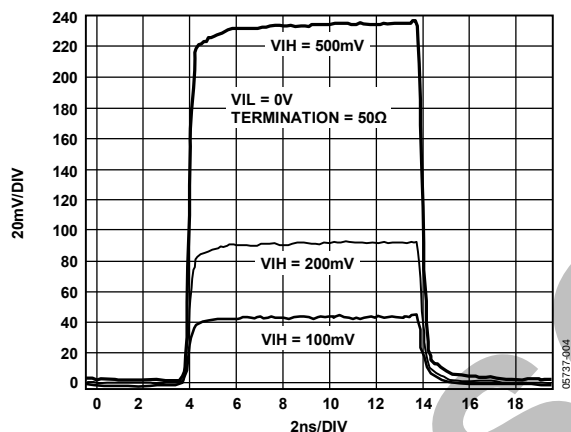
Figure 4. Driver Small Signal Response
