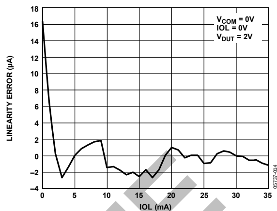
Figure 17. Active Load Linearity vs. IOH
