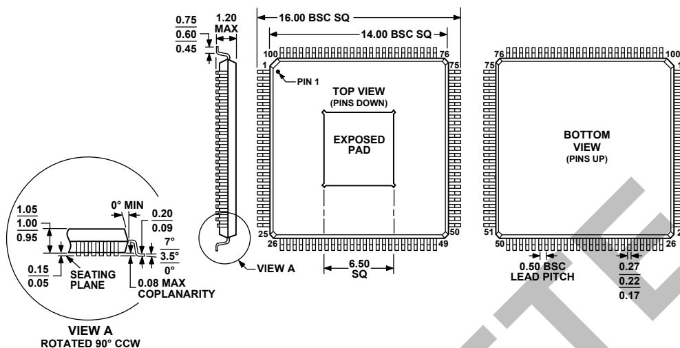
Figure 19. 100-Lead Thin Quad Flat Package, Exposed Pad [TQFP_EP] (SV-100-2)
