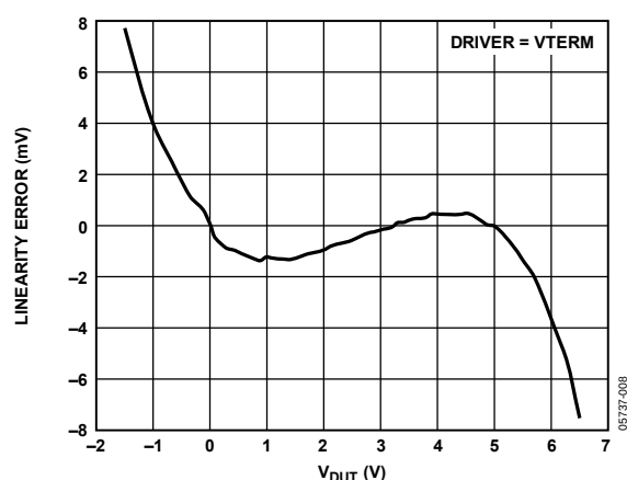
Figure 8. Driver VTERM Linearity vs. Output
