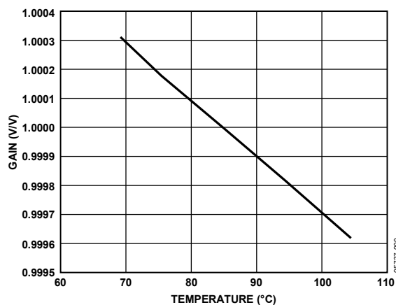
Figure 9. Driver Gain vs. Temperature
