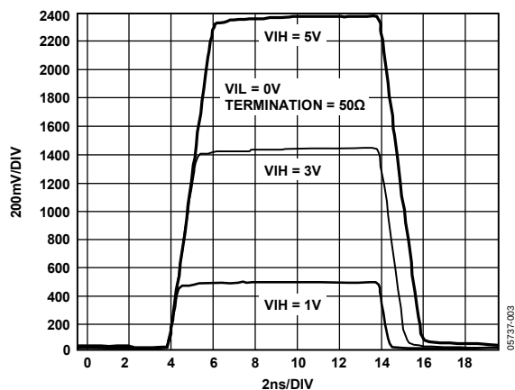
Figure 3. Driver Large Signal Response
