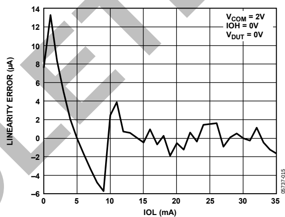
Figure 18. Active Load Linearity vs. IOL
