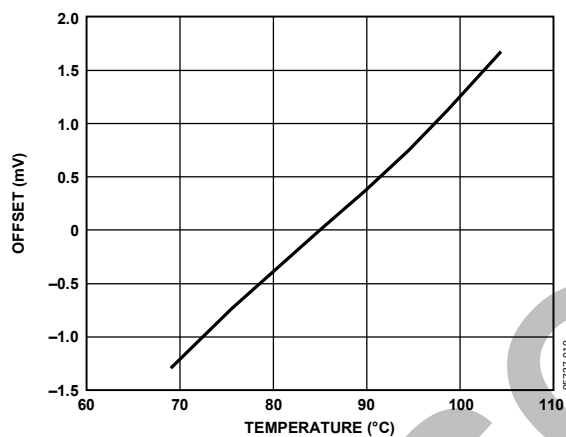
Figure 10. Driver Offset vs. Temperature
