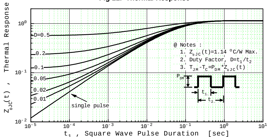
Fig 11. Thermal Response
