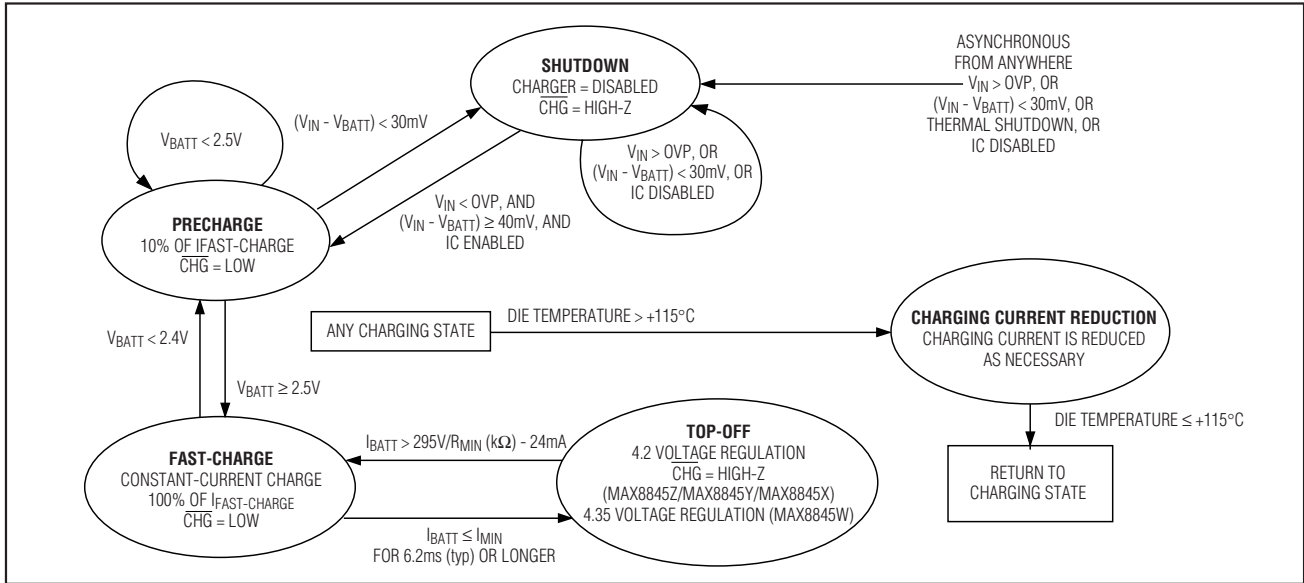
Figure 2. Charge-State Diagram
