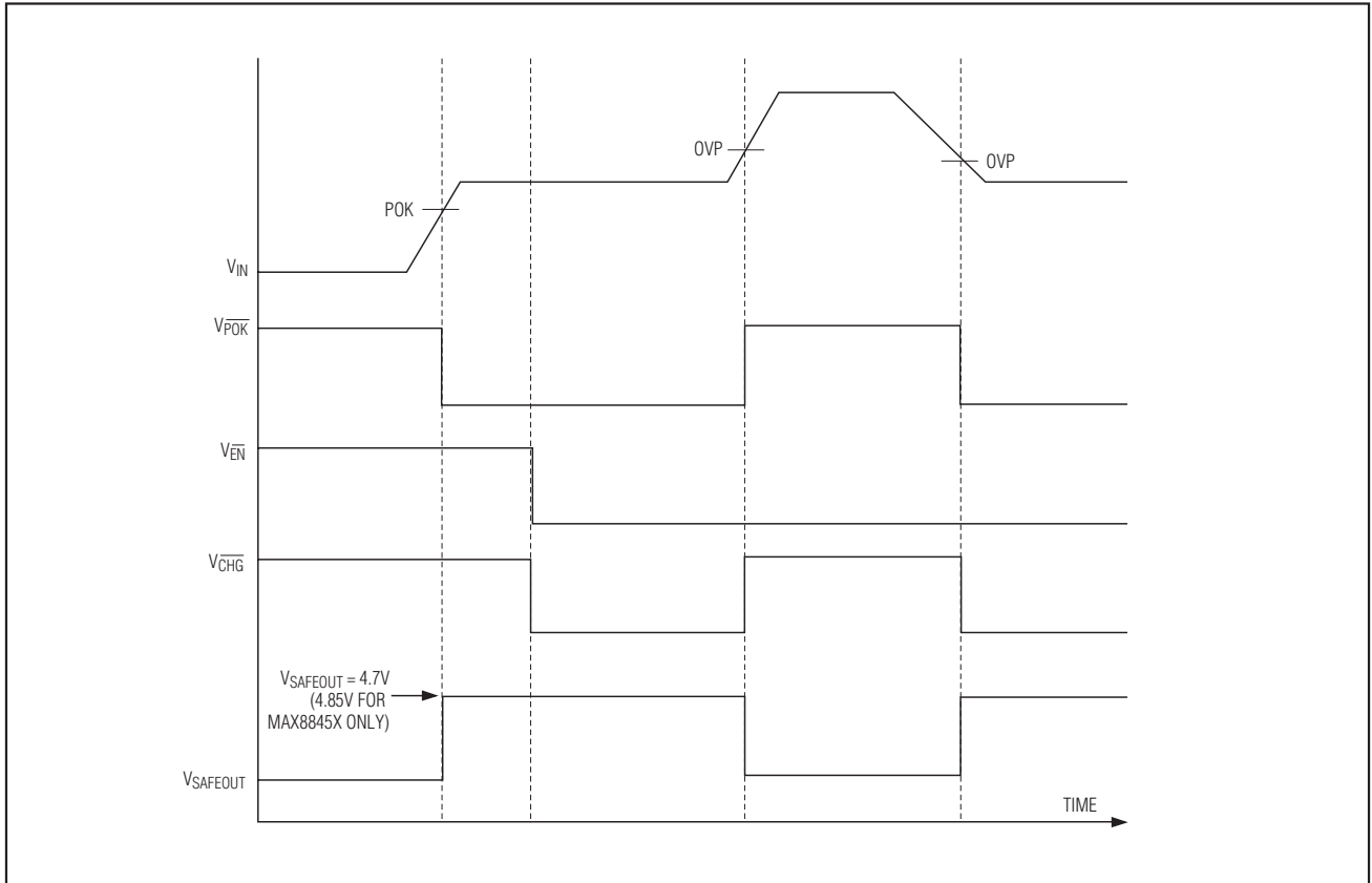
Figure 6. Timing Diagram
