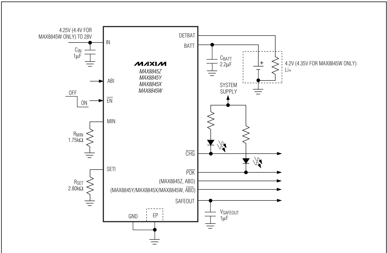
Typical Operating Circuit
