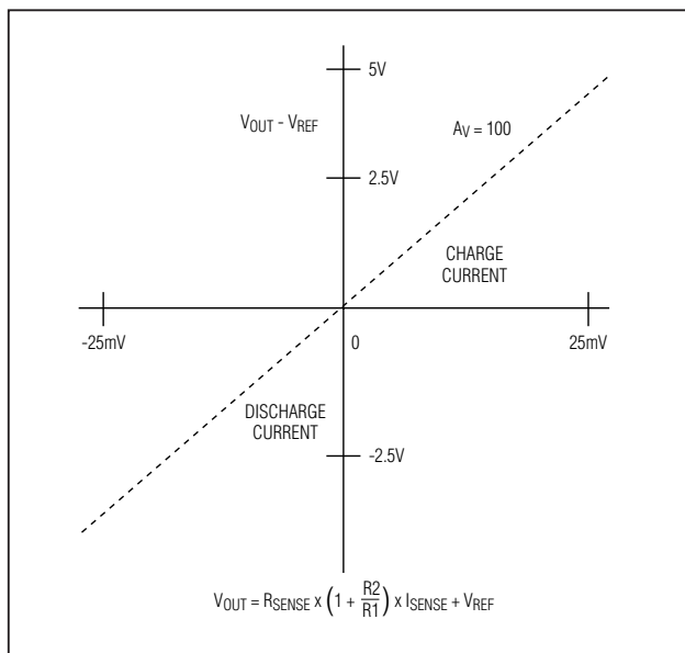
Figure 1. Bidirectional Current-Sense Transfer Function
