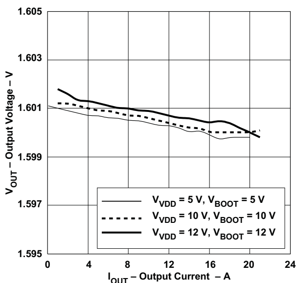
Figure 1. Load Regulation
