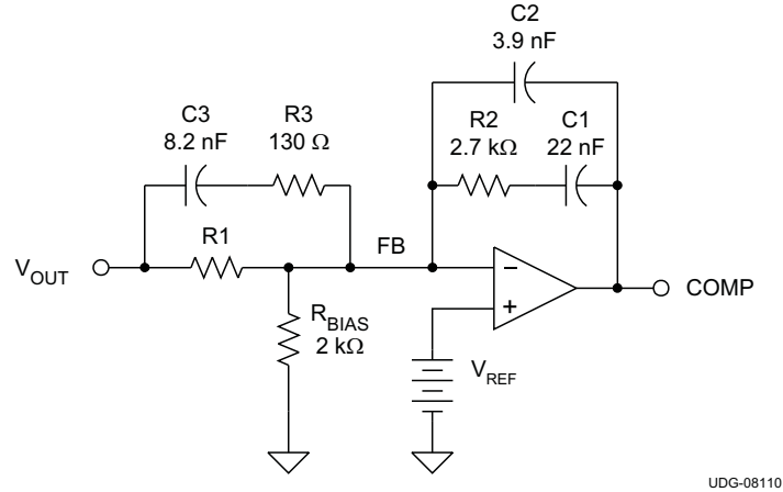
Figure 10. Parameters for Type III Compensation Network
