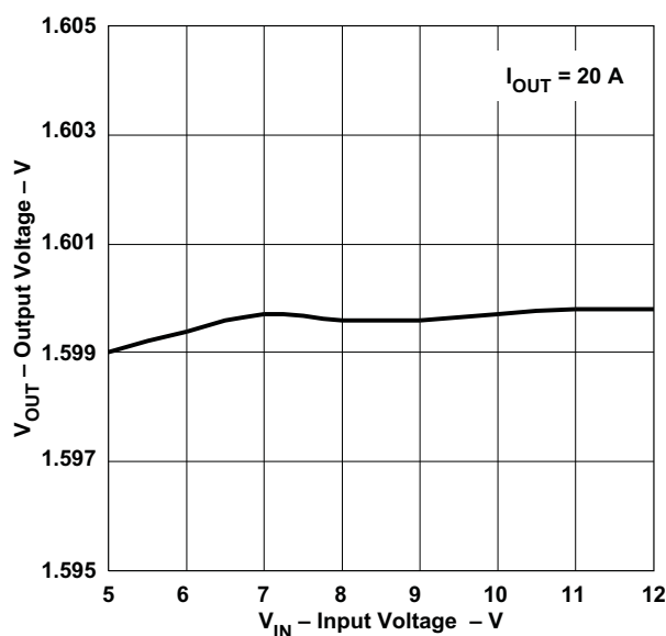
Figure 2. Line Regulation
