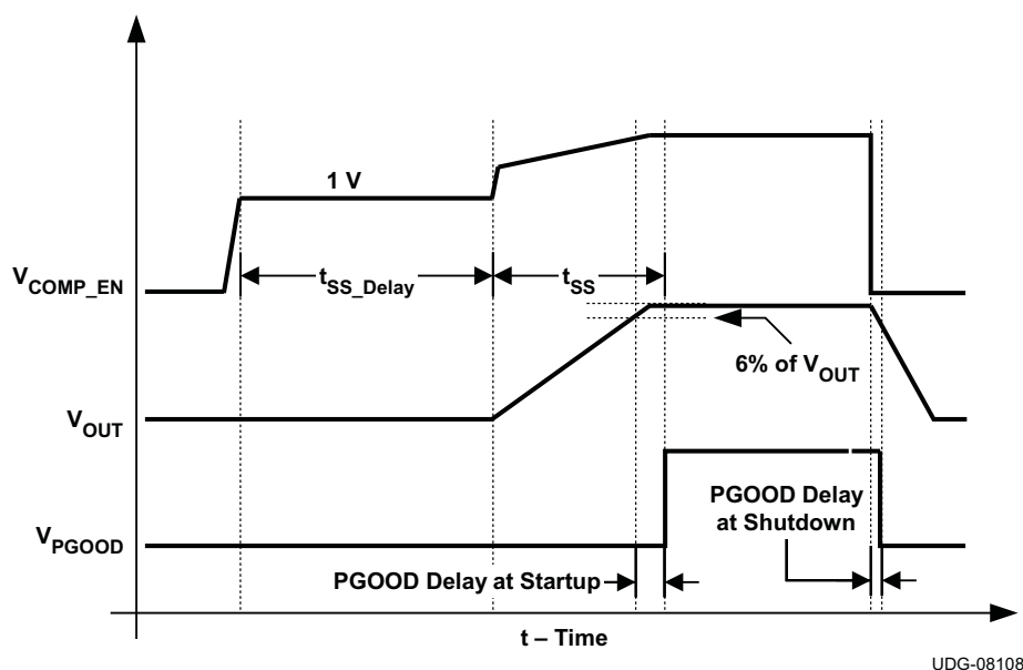
Figure 7. Typical Startup and Shutdown Sequence
