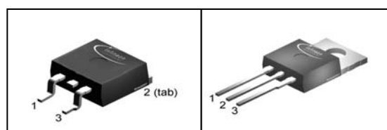
PG-TO263-3-2
