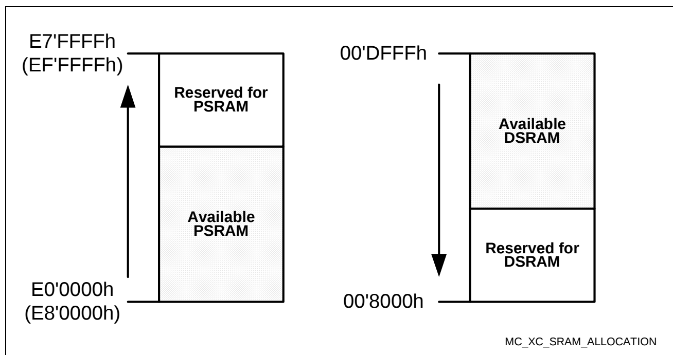
Figure 1 SRAM Allocation
