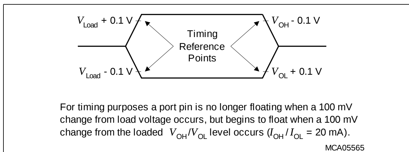
Figure 18 Floating Waveforms
