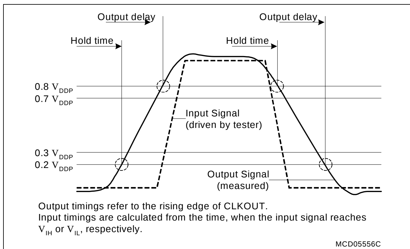
Figure 17 Input Output Waveforms
