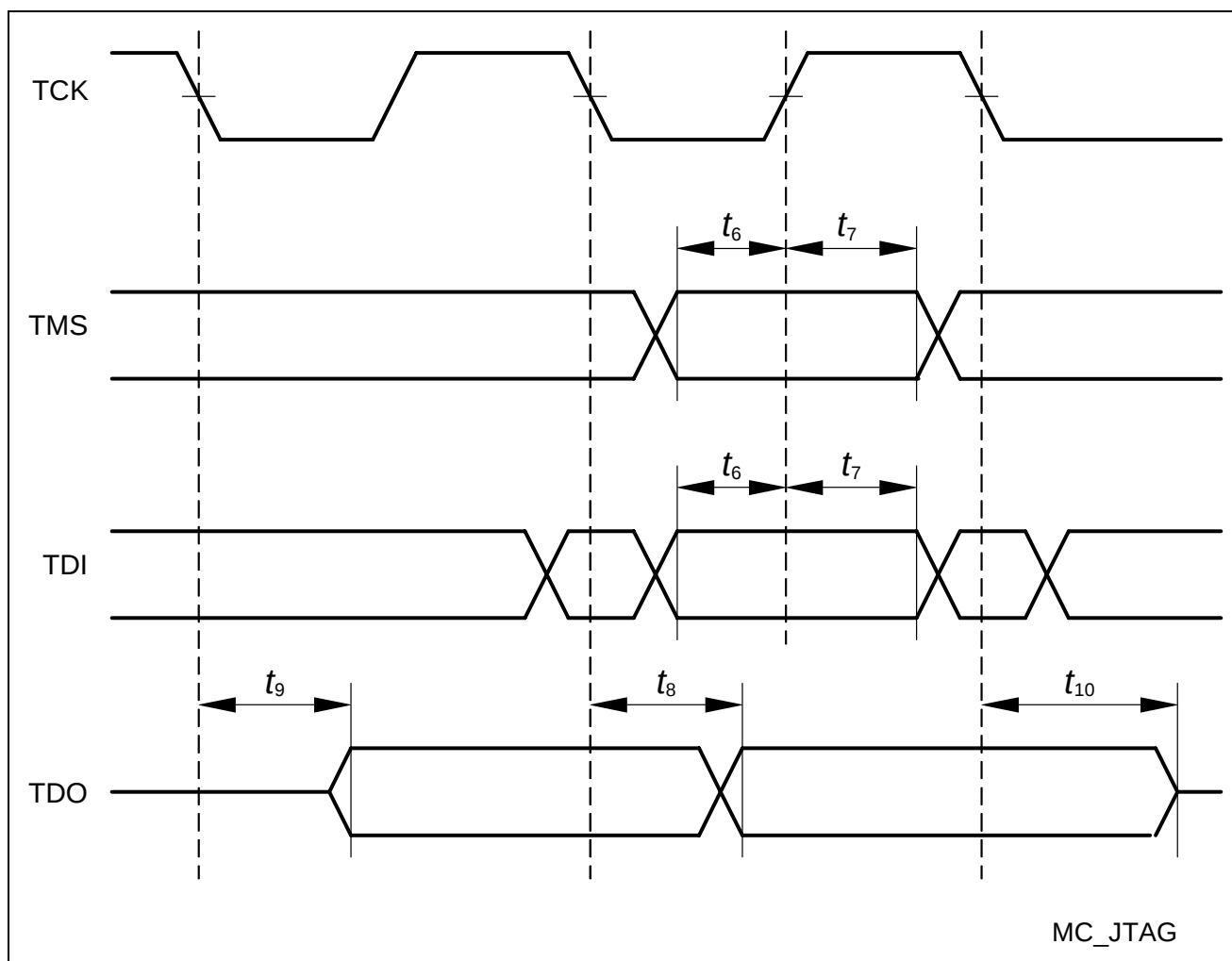
Figure 31 JTAG Timing
