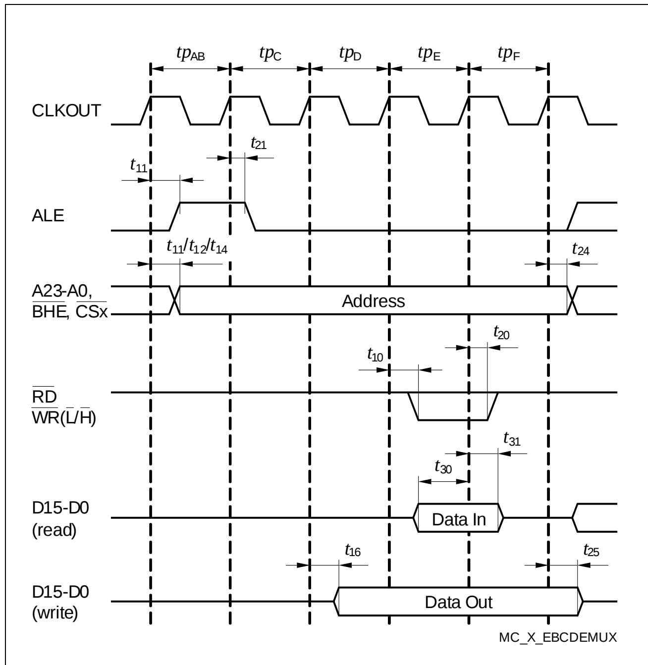
Figure 24 Demultiplexed Bus Cycle
