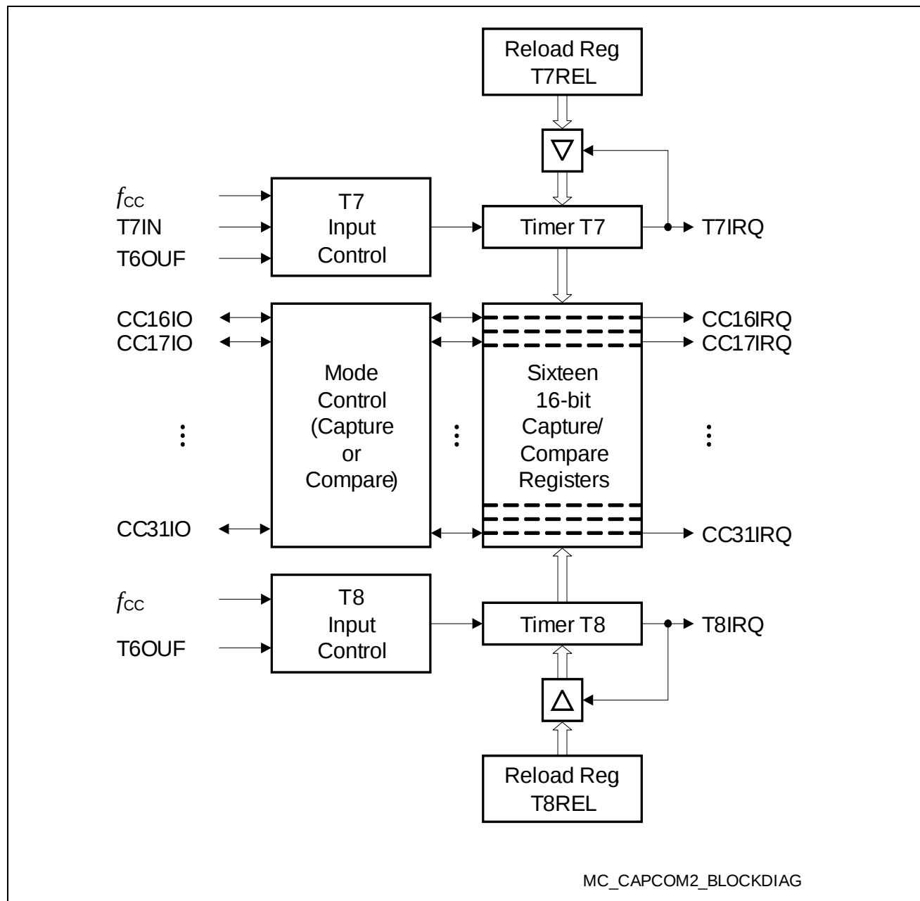
Figure 6 CAPCOM2 Unit Block Diagram
