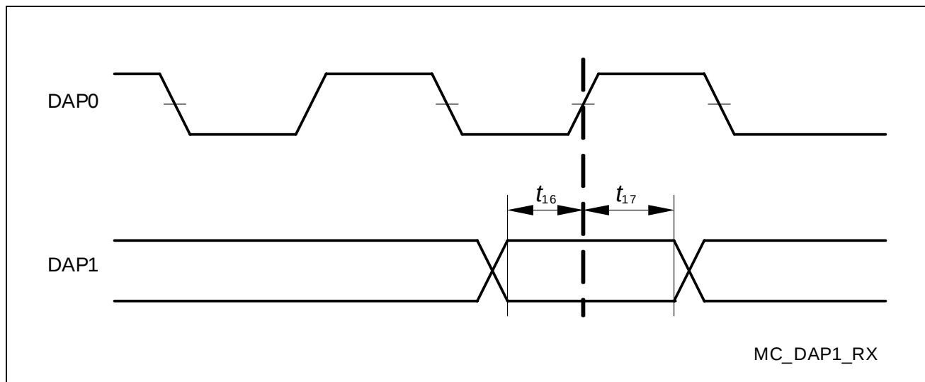
Figure 28 DAP Timing Host to Device
