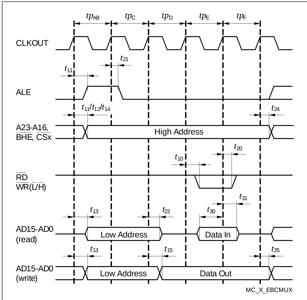
Figure 23 Multiplexed Bus Cycle
