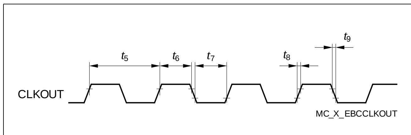
Figure 22 CLKOUT Signal Timing
