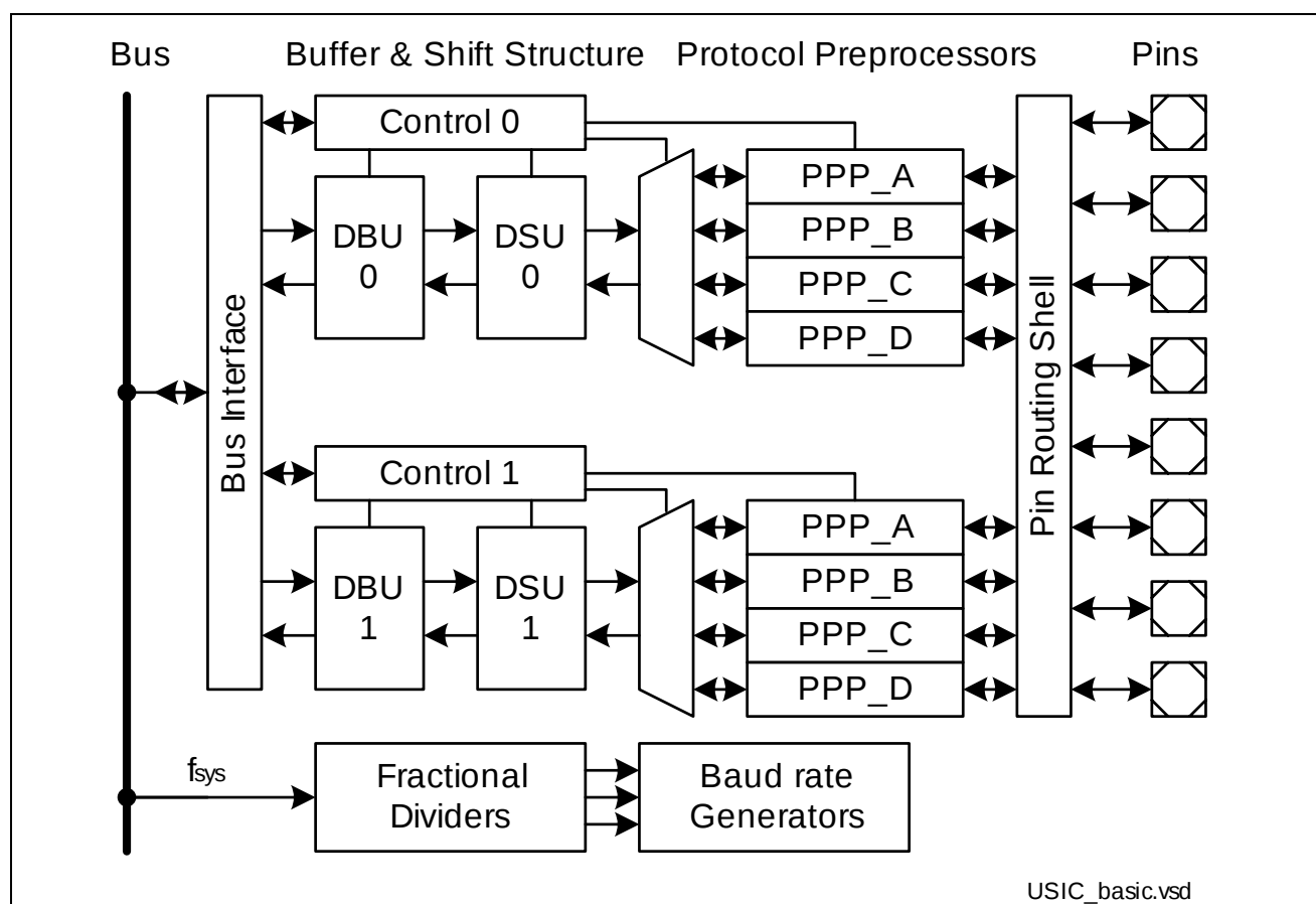
Figure 11 General Structure of a USIC Module
