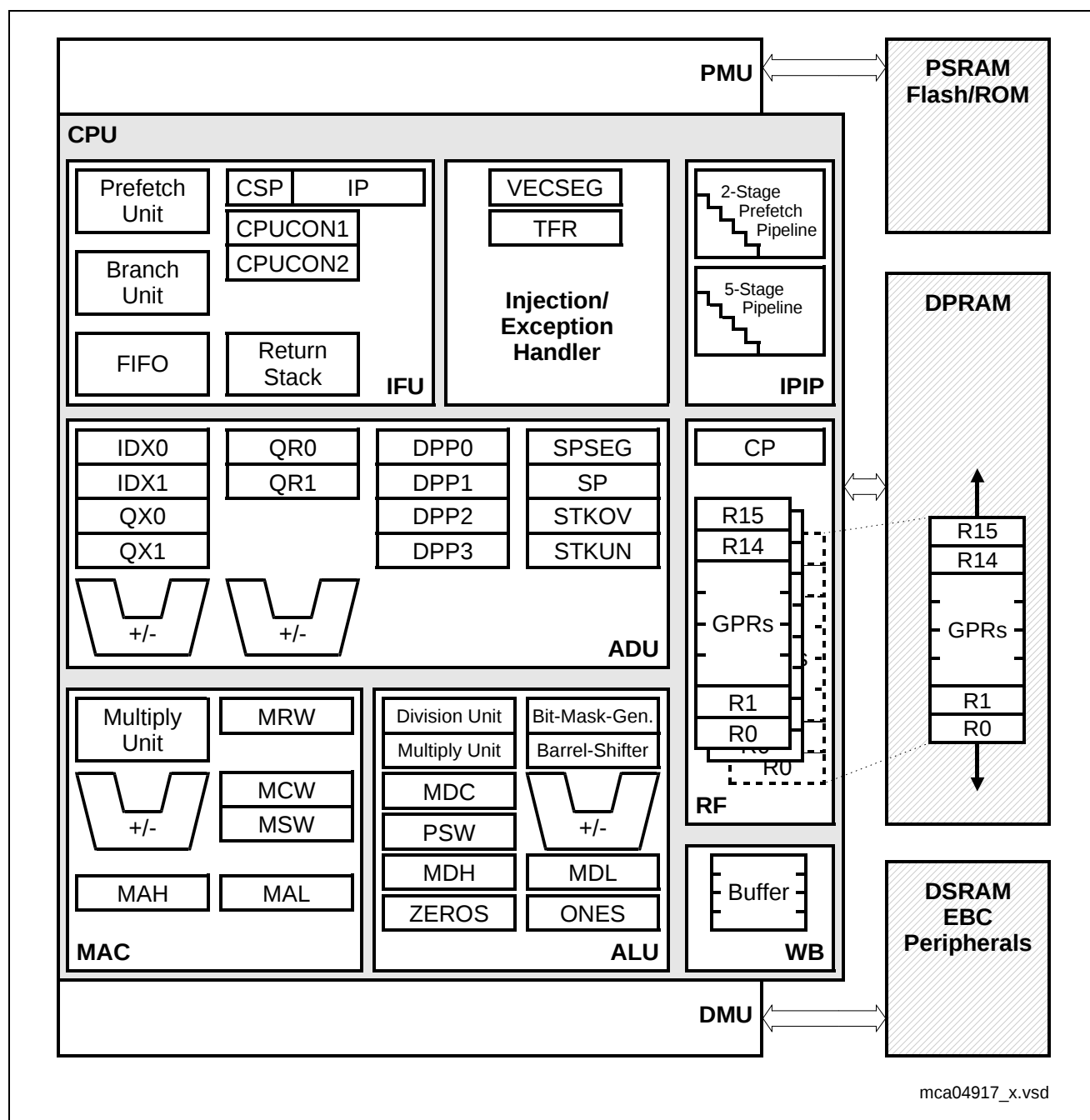
Figure 5 CPU Block Diagram
