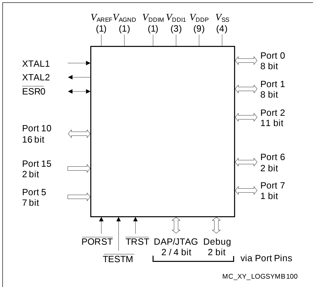
Figure 2 XC2765X Logic Symbol
