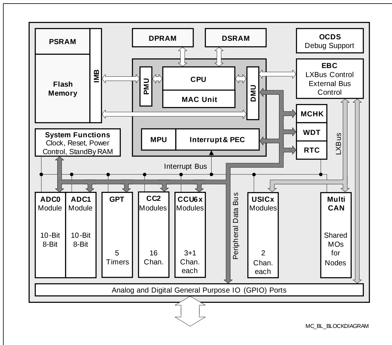
Figure 4 Block Diagram
