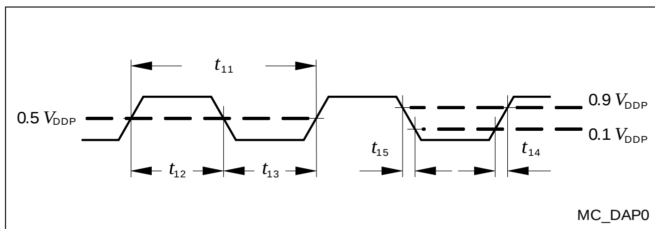
Figure 27 Test Clock Timing (DAP0)
