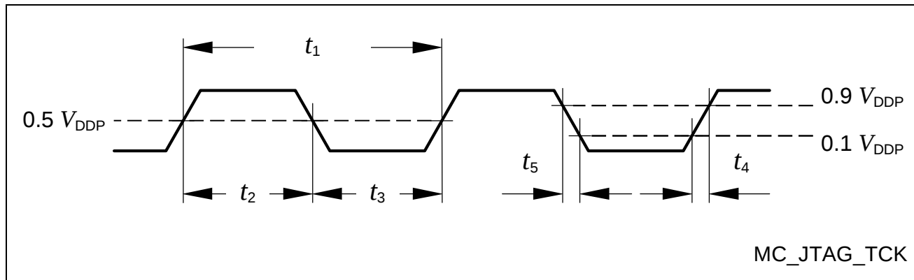
Figure 30 Test Clock Timing (TCK)
