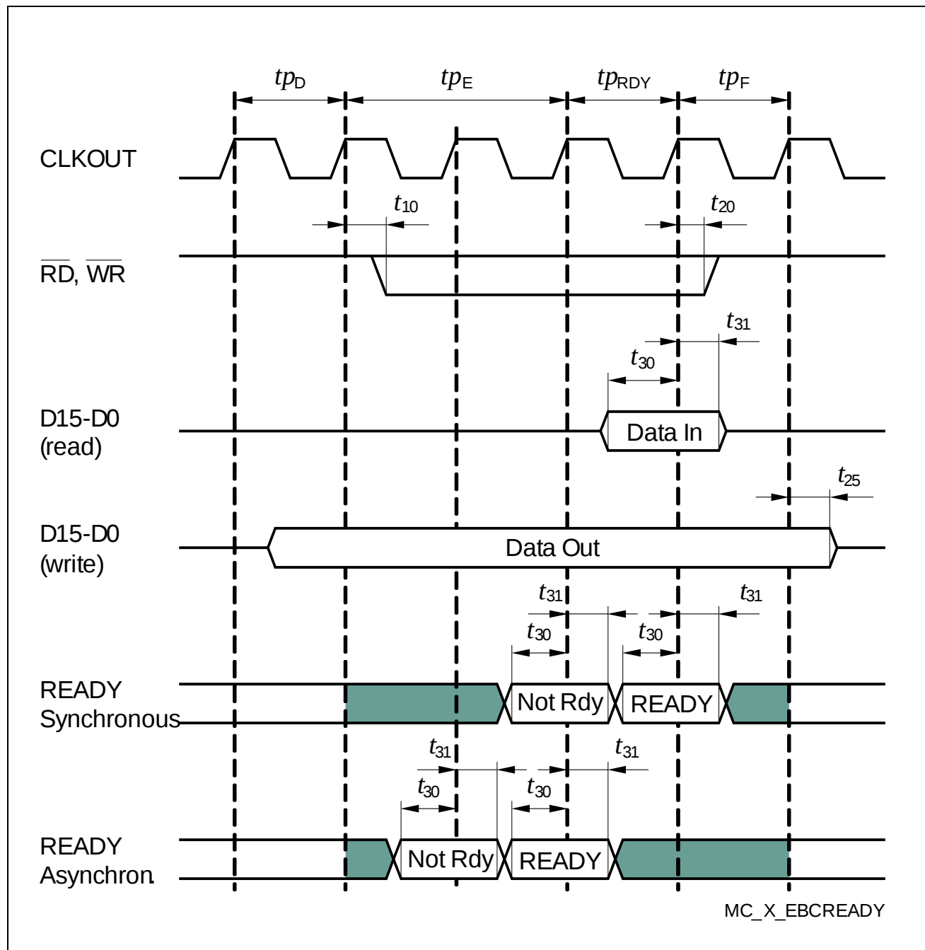
Figure 25 READY Timing
