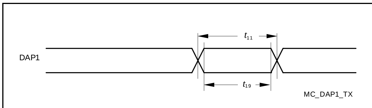
Figure 29 DAP Timing Device to Host
