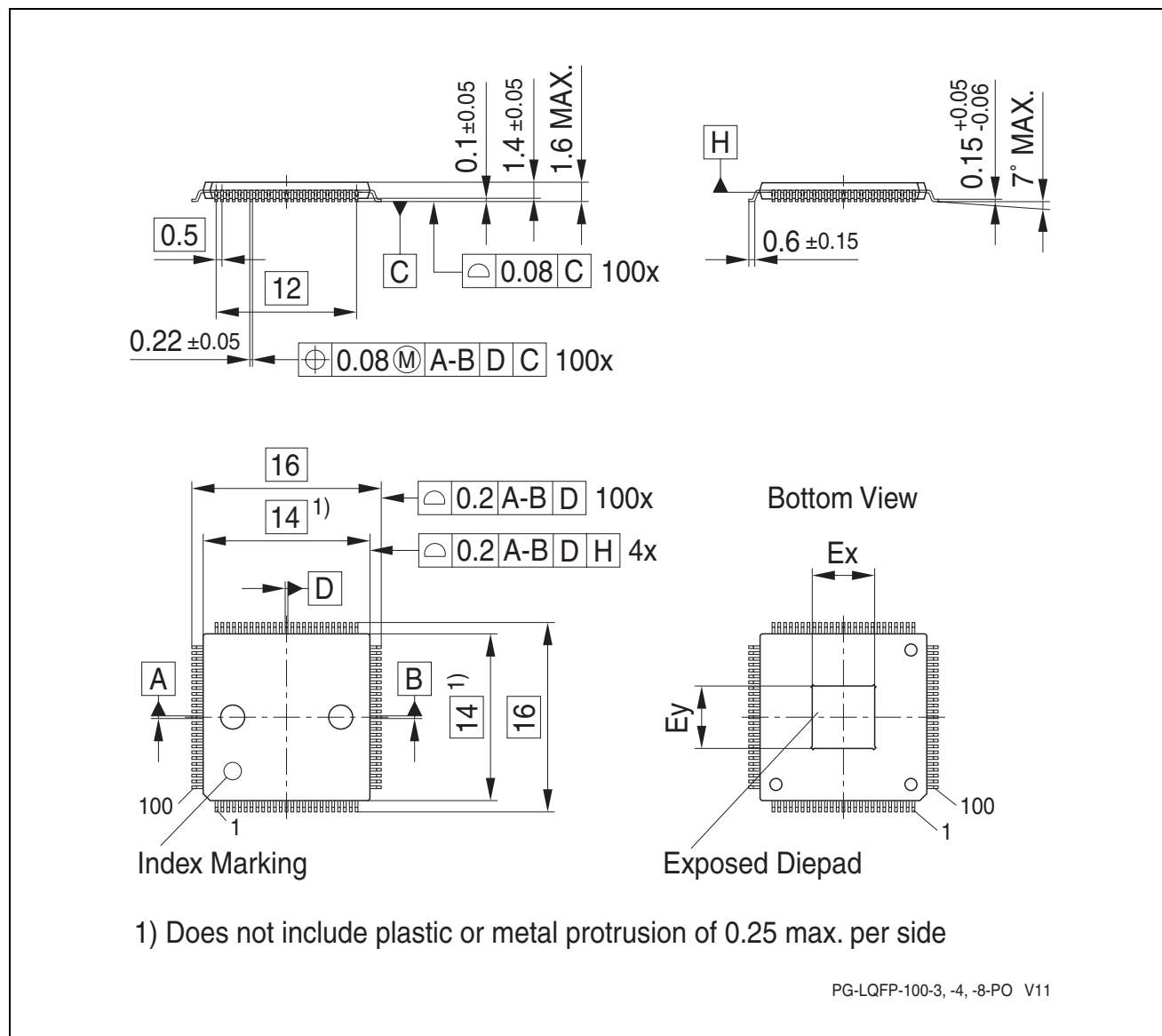
Figure 32 PG-LQFP-100-8 (Plastic Green Thin Quad Flat Package)
