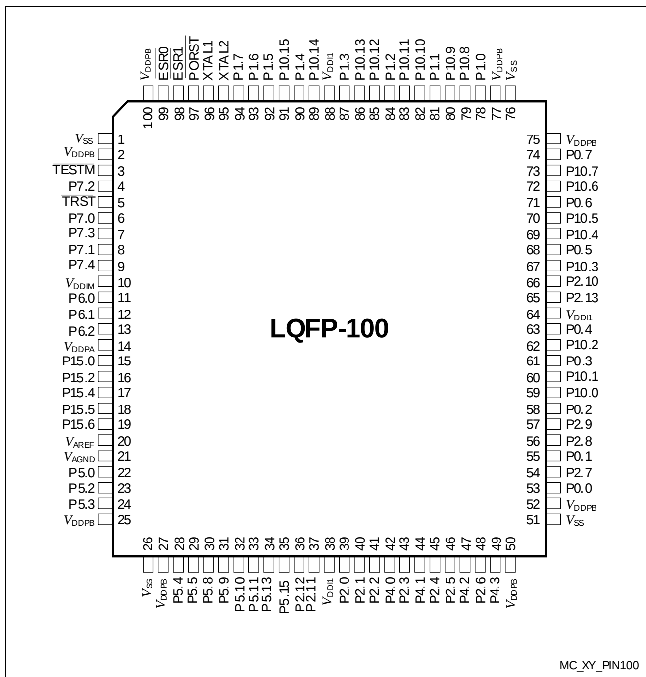
Figure 3 XC2765X Pin Configuration (top view)
