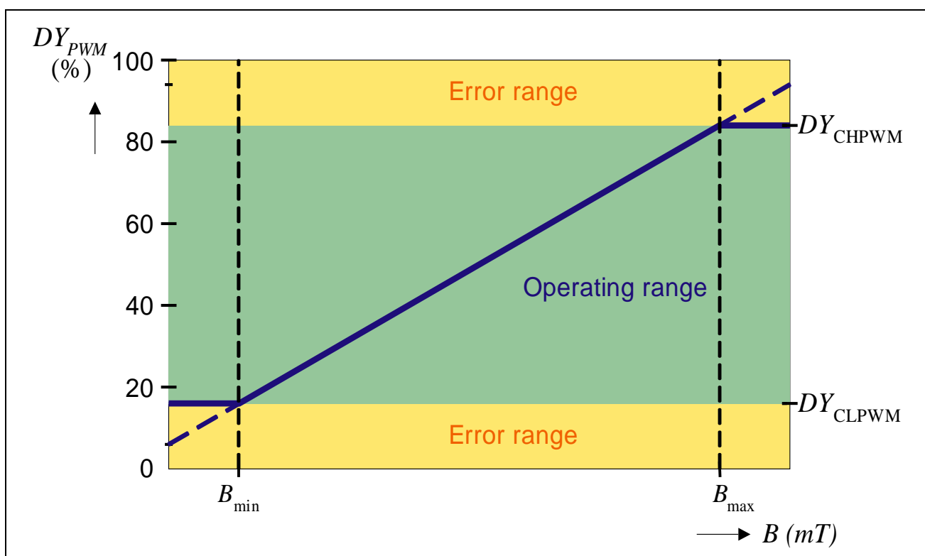
Figure 8 Clamping example
