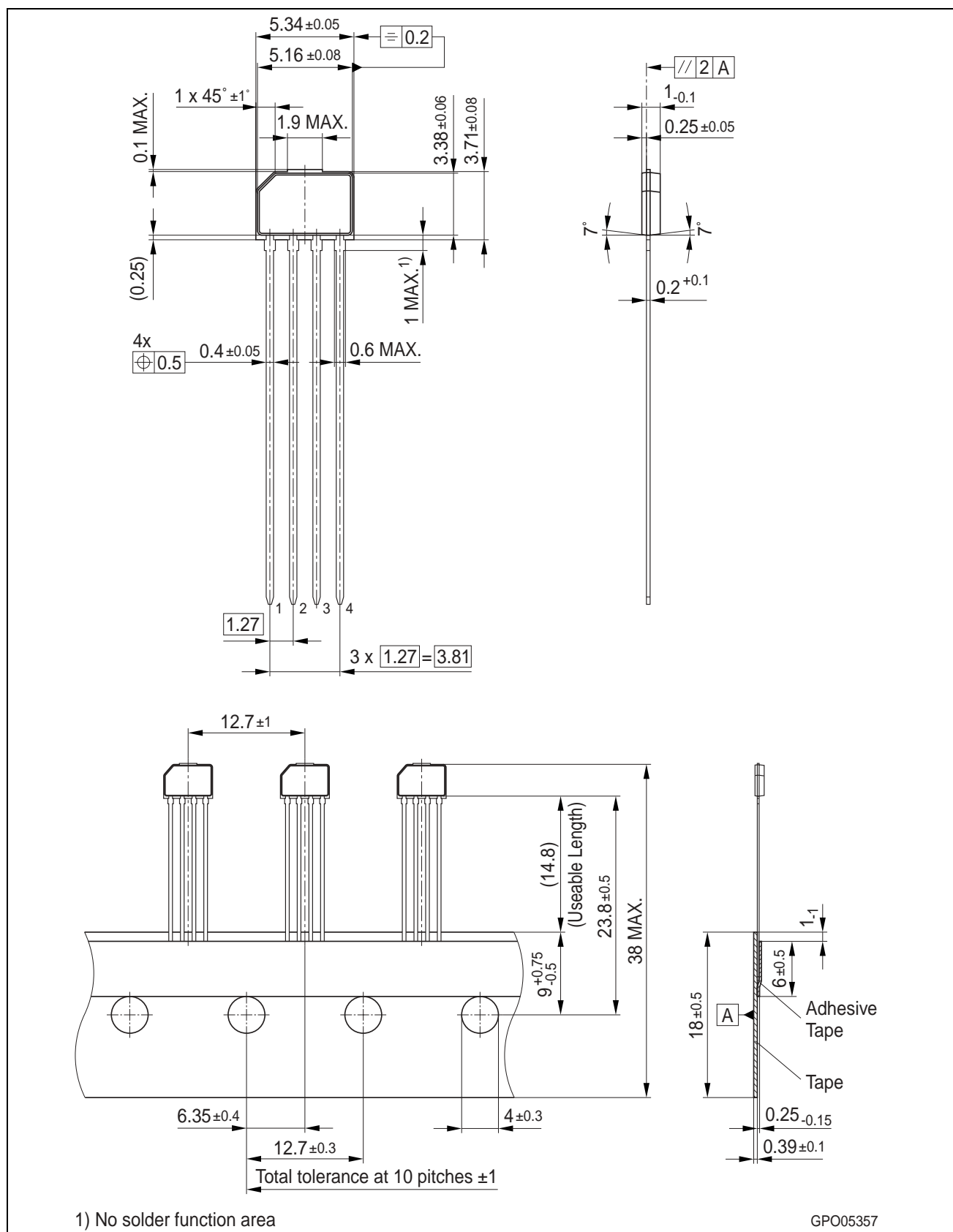
Figure 12 PG-SSO-4-1 (Plastic Green Single Small Outline Package)
