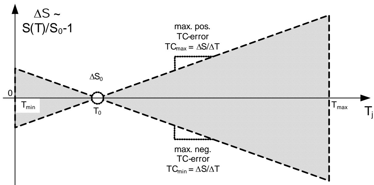
Figure 5 Drift of temperature coefficient
