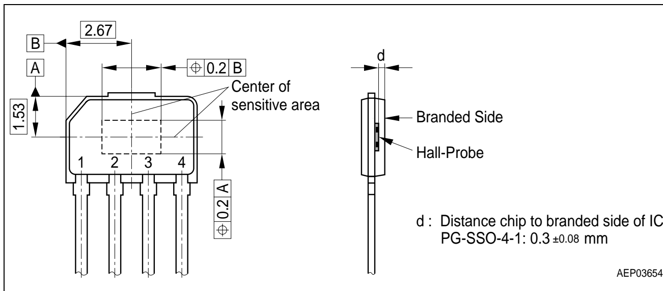
Figure 2 TLE4998P4 Pin Configuration and Hall Cell Location
