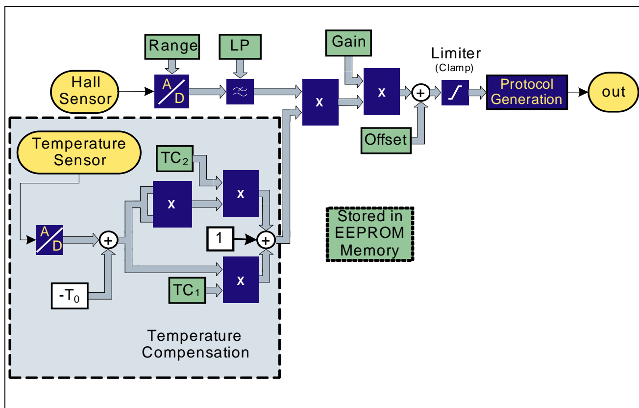
Figure 6 Signal Processing Flow
