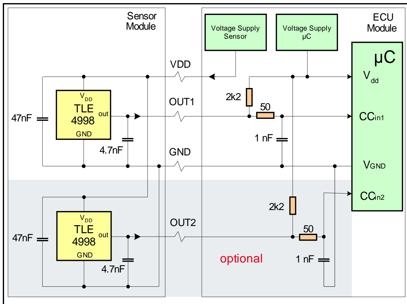
Figure 10 Application Circuit
