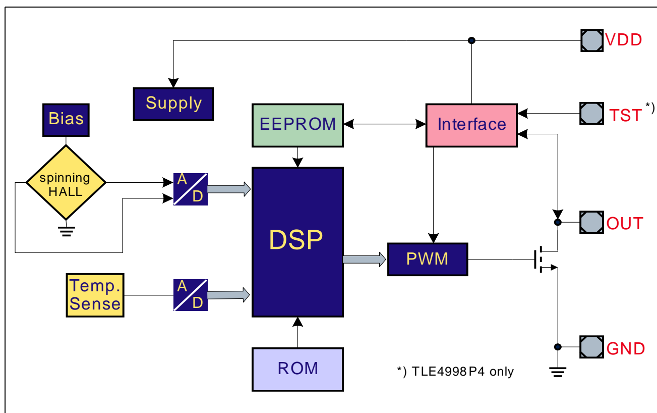
Figure 3 Block Diagram
