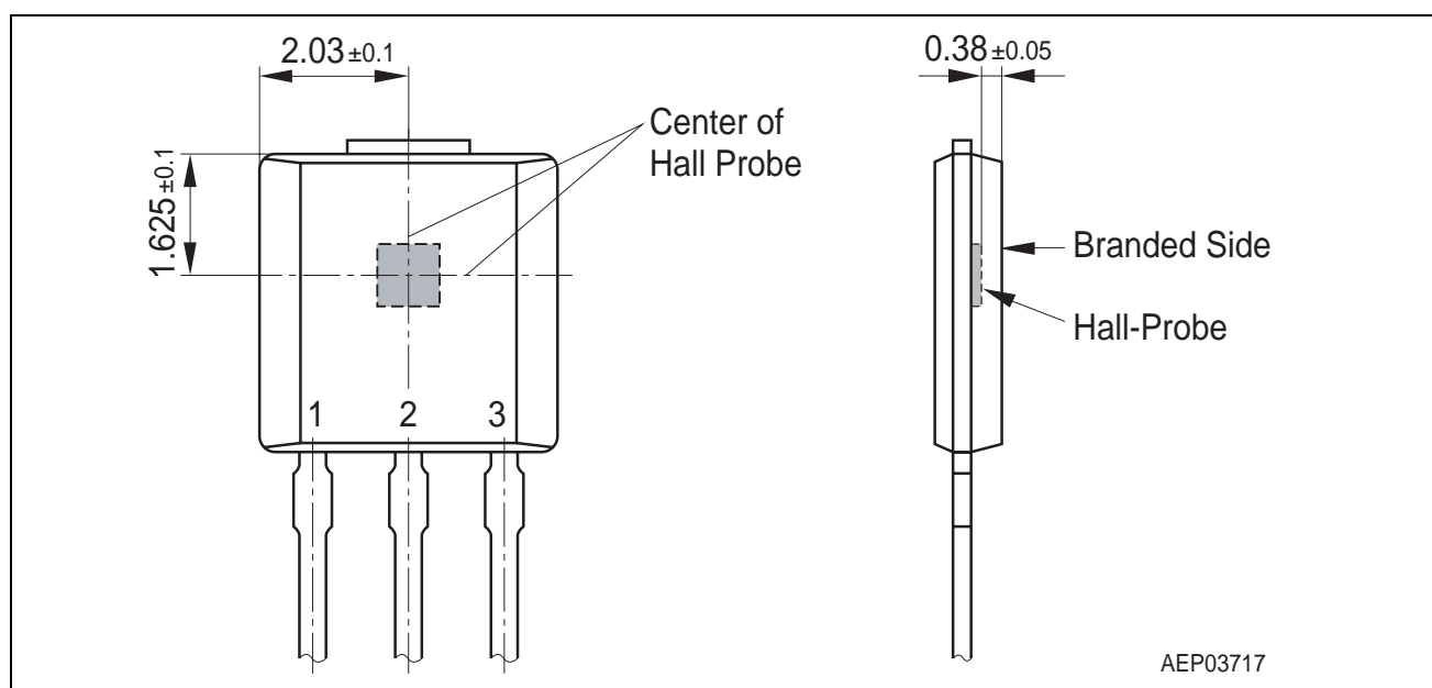
Figure 1 TLE4998P3 Pin Configuration and Hall Cell Location
