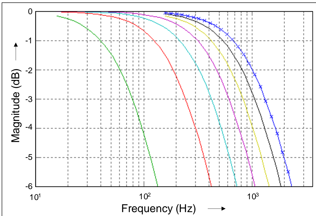
Figure 7 DSP Input Filter (Magnitude Plot)
