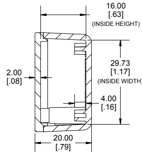
END VIEW SECTION B-B
