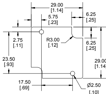
MAXIMUM P.C. BOARD SIZE
