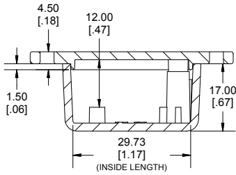
SIDE VIEW SECTION A-A
