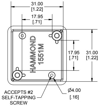
INSIDE BOX
