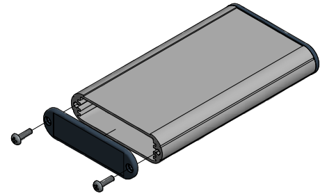
EXPLODED ASSEMBLY VIEW
