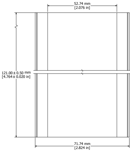
EXTRUSION
