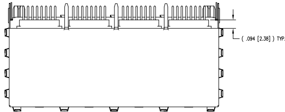
PIN DETAIL TYP. ALL PORTS
