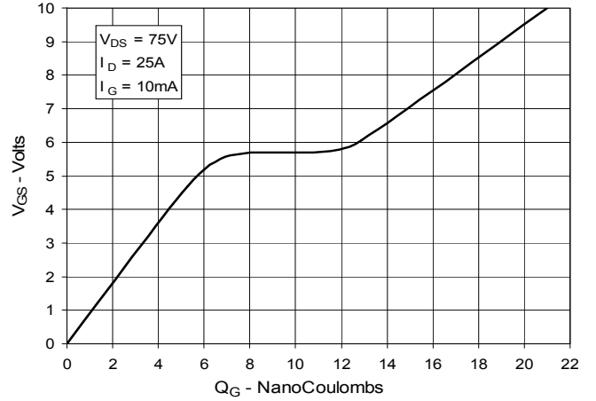
Fig. 10. Gate Charge
