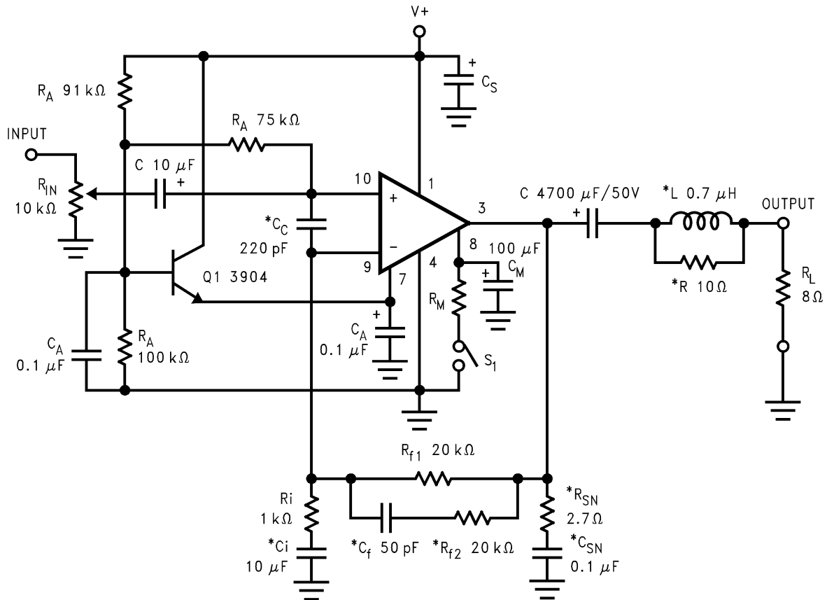
Figure 3. Typical Single Supply Audio Amplifier Application Circuit
