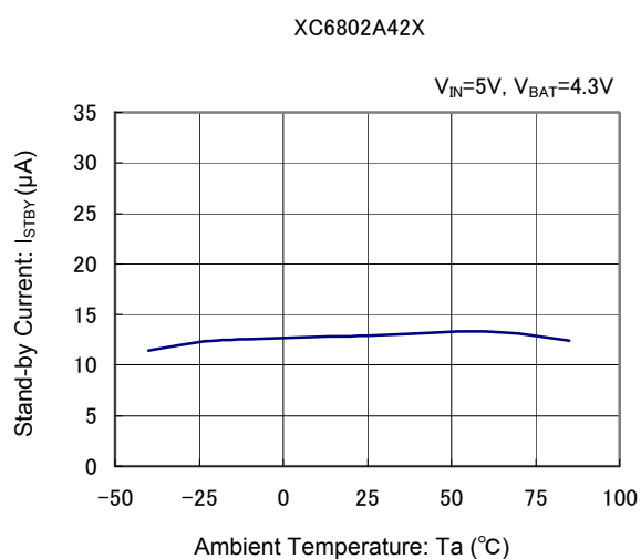
(17) Stand-by Current vs. Ambient Temperature
