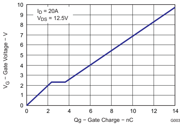
Figure 4. Gate Charge
