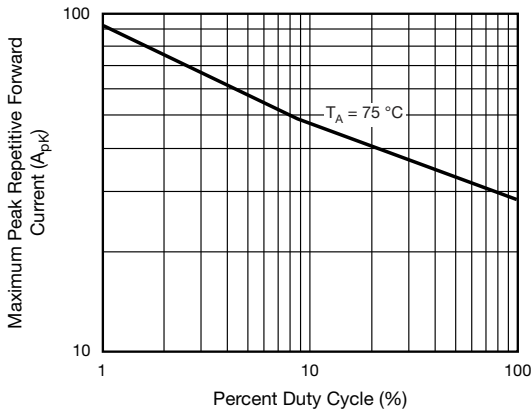
Fig. 3 - Maximum Peak Repetitive Forward Surge Current
