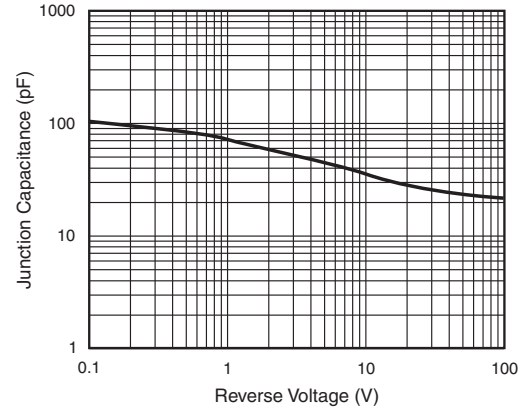
Figure 5. Typical Capacitance
