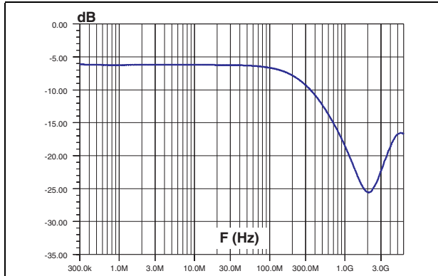
Figure 5. S21(db) attenuation (DATA line)
