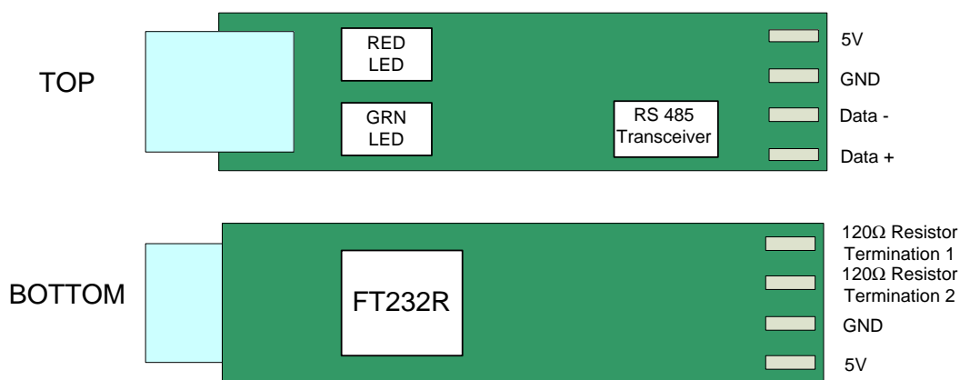
USB-RS485-PCB Rev 2
