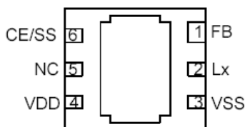
USP-6C (BOTTOM VIEW)
