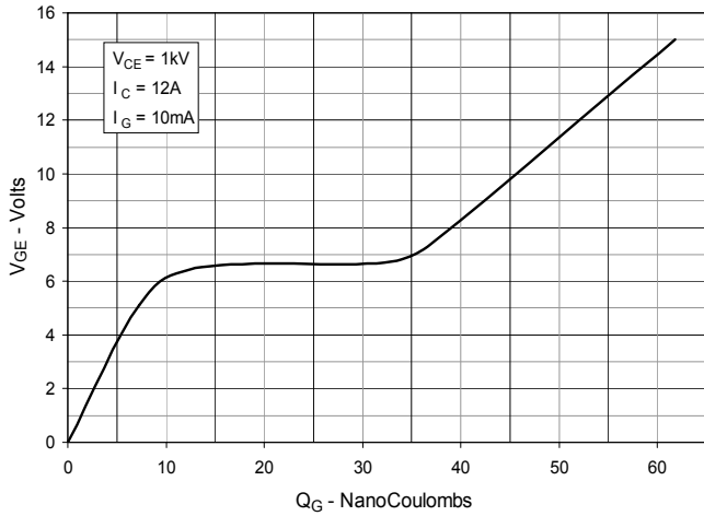
Fig. 9. Gate Charge
