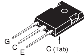
TO-247 (IXBH)
