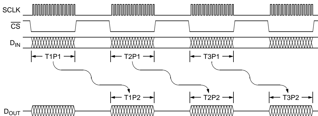
Figure 4-2 Single-Level Communications Queuing Detail
