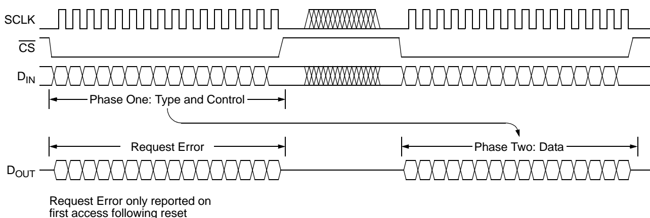
Figure 4-1 Transfer Phase Detail
