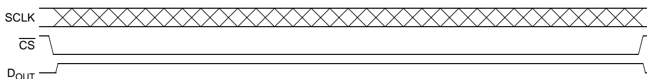
Figure 4-17 Oscillator Failure Response
