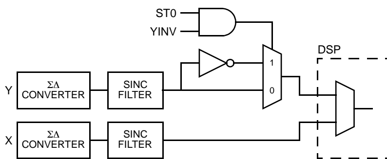
Figure 3-1 Y-Axis Inversion Function
