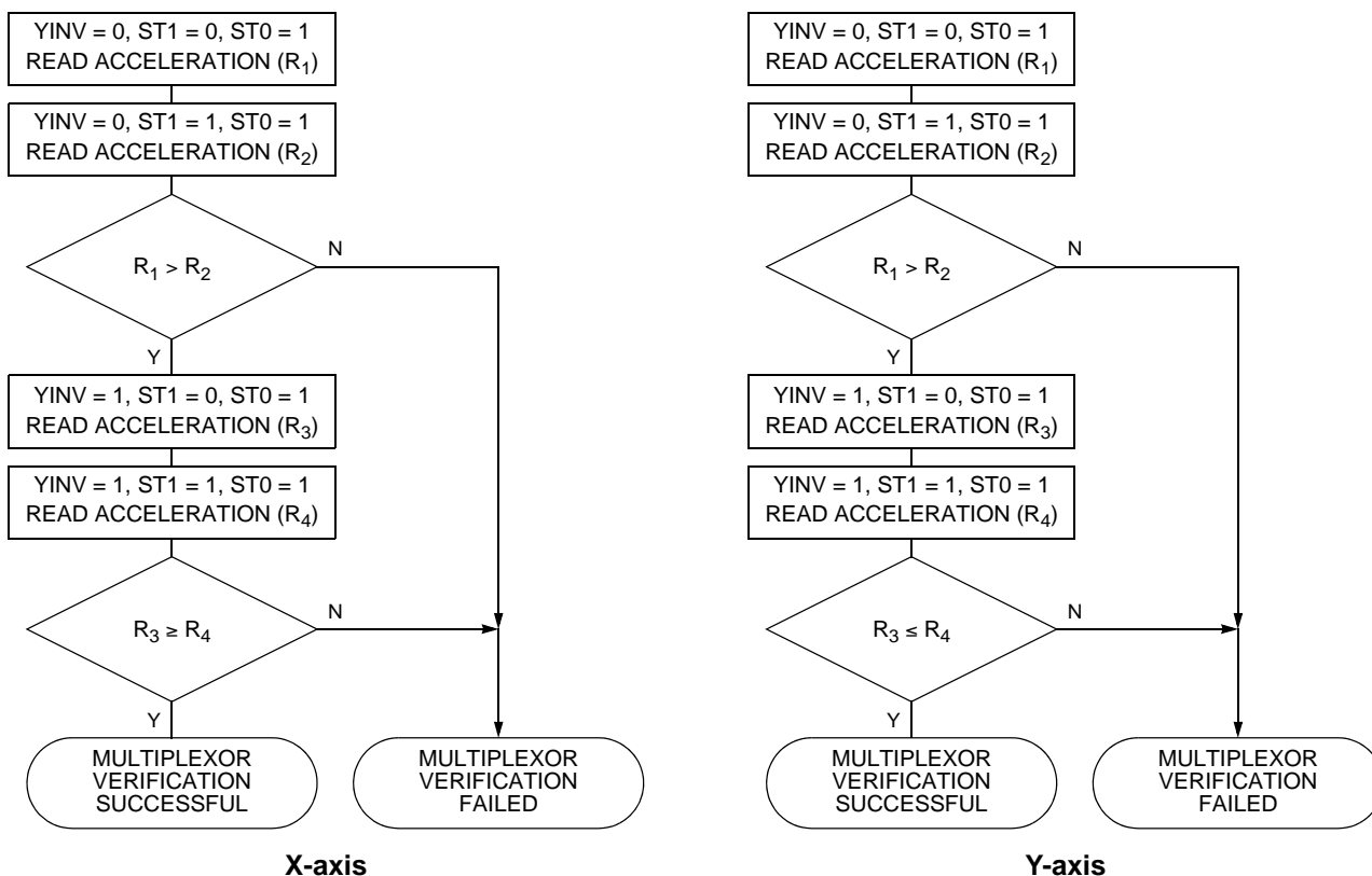
Figure 3-2 DSP Input Multiplexor Verification Flow Chart
