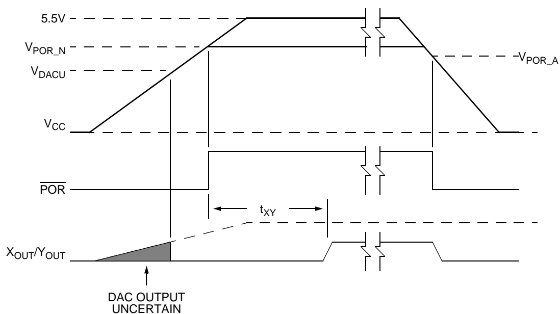
Figure 2-1 Power-Up Timing
