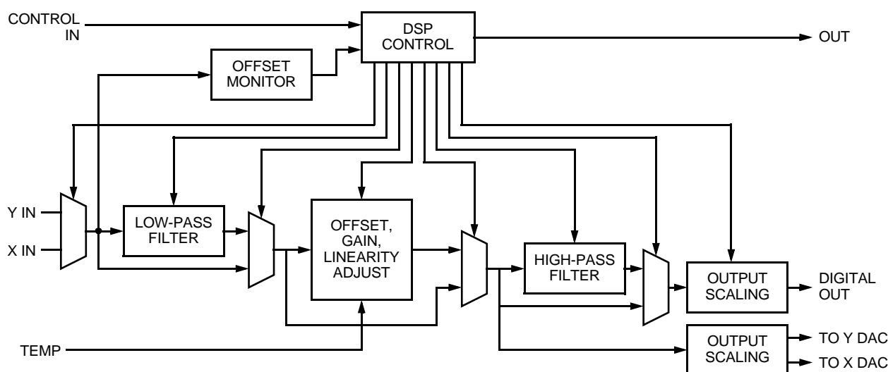
Figure 1-2 MMA62XXEG Block Diagram
