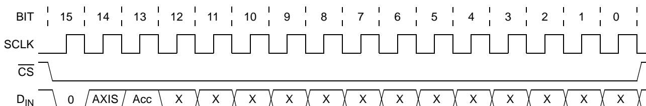
Figure 4-4 Acceleration Command Format
