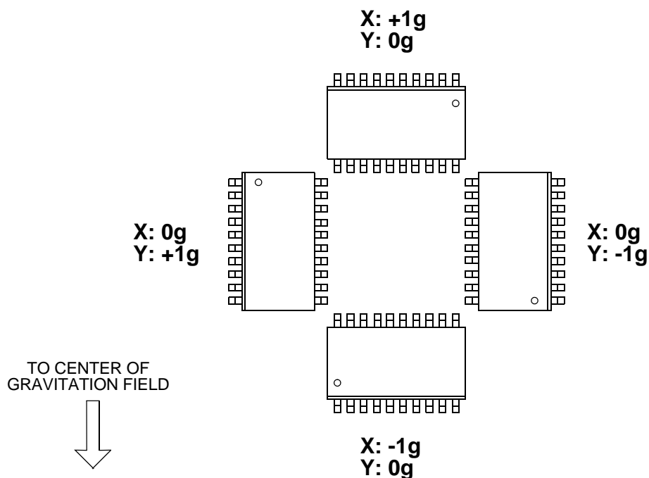
Response to static orientation within 1g field.
