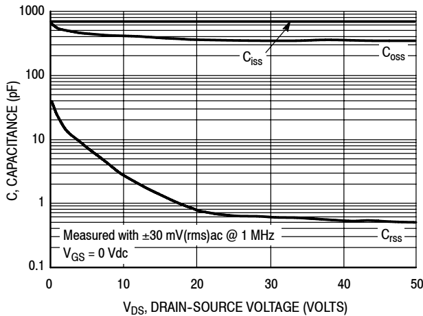
Figure 3. Capacitance versus Drain-Source Voltage
