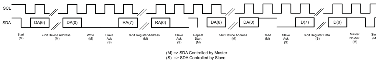
Figure 5-33. I 2 C Read
