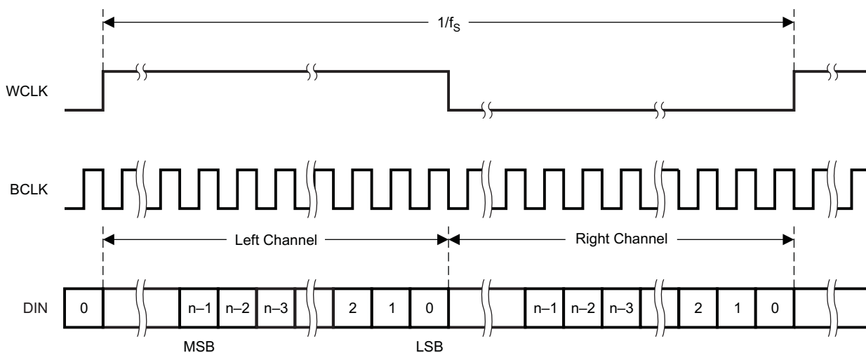
Figure 5-21. Timing Diagram for Right-Justified Mode
