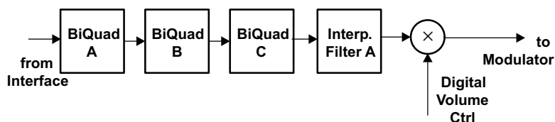
Figure 5-2. Signal Chain for PRB_P4
