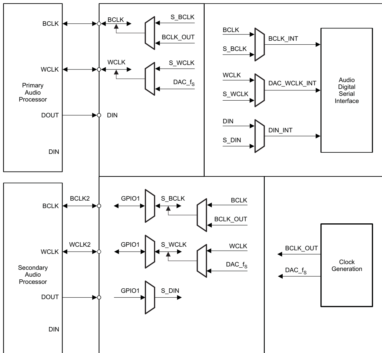
Figure 5-31. Audio Serial Interface Multiplexing
