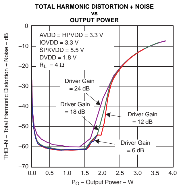
Figure 4-4. Max Class-D Speaker-Driver Output Power ( R_L = 4 \Omega )
