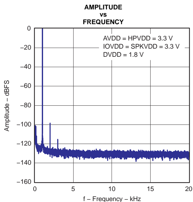
Figure 4-8. FFT - Line In Bypass to Line Output
