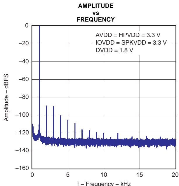
Figure 4-2. FFT - DAC to Headphone Output
