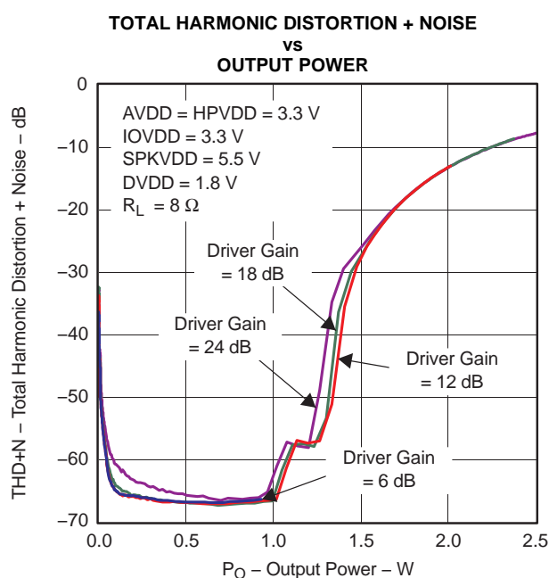
Figure 4-6. Max Class-D Speaker-Driver Output Power ( R_L = 8 \Omega )
