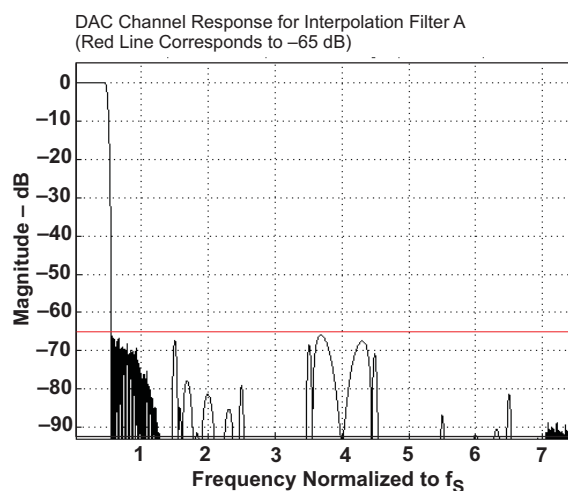
Figure 5-12. Frequency Response of DAC Interpolation Filter A
