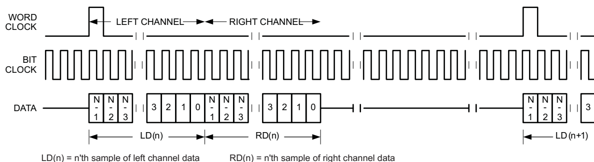
Figure 5-28. Timing Diagram for DSP Mode
