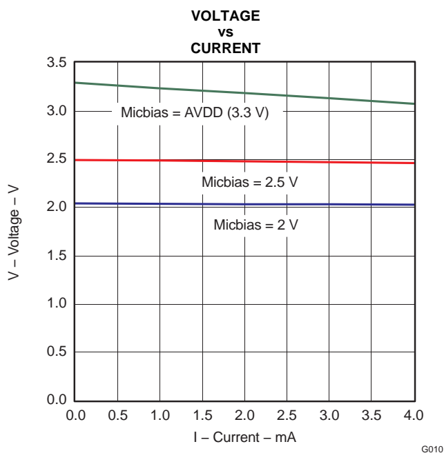
Figure 4-10. MICBIAS
