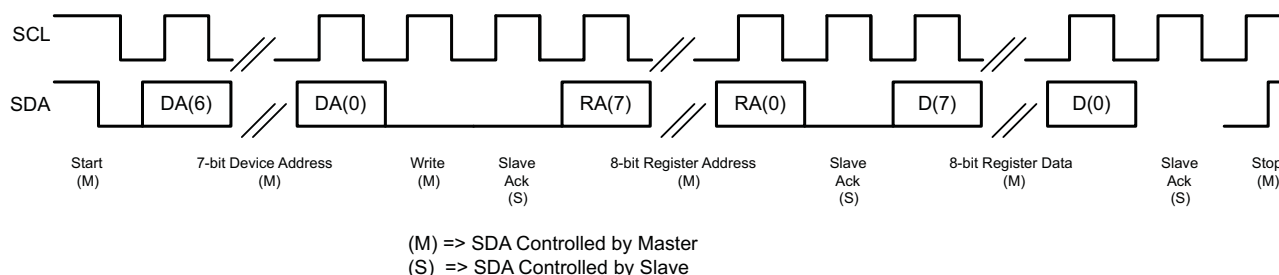
Figure 5-32. I 2 C Write
