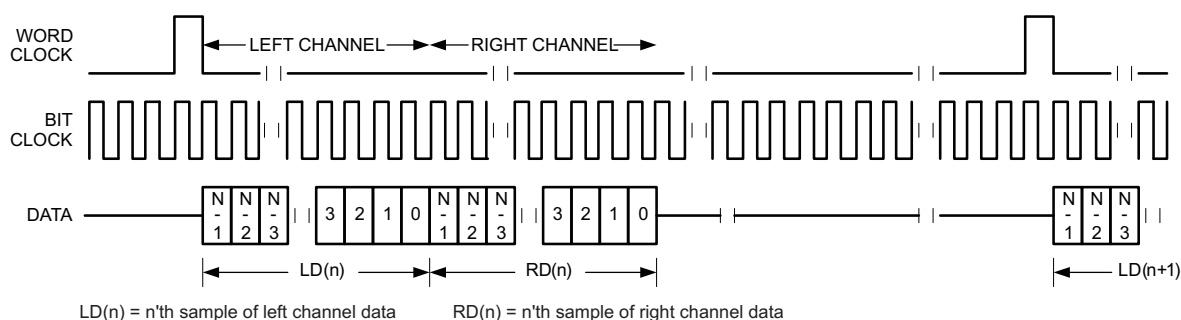
Figure 5-29. Timing Diagram for DSP Mode With Offset = 1
