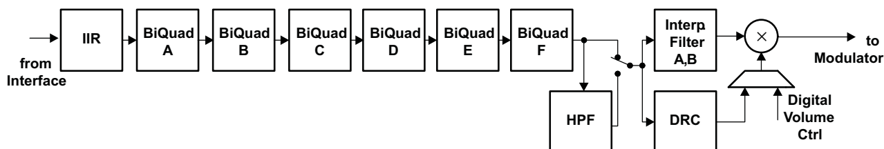
Figure 5-3. Signal Chain for PRB_P5 and PRB_P15
