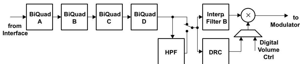
Figure 5-6. Signal Chain for PRB_P13
