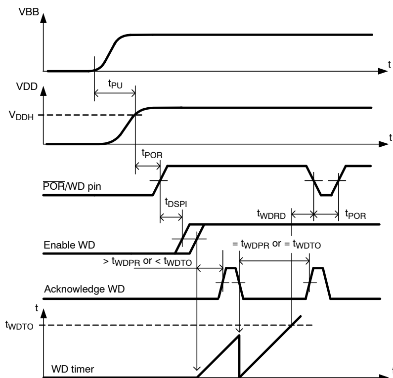
Figure 15. Watchdog Timing Diagram
