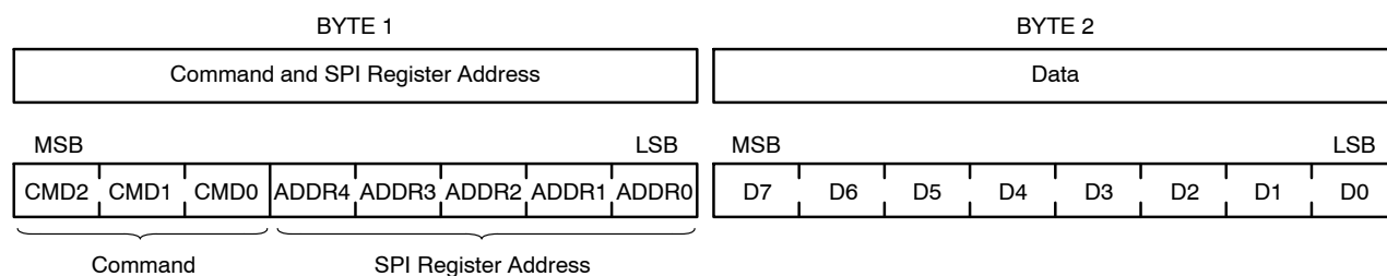
Figure 17. SPI Transfer Packet
