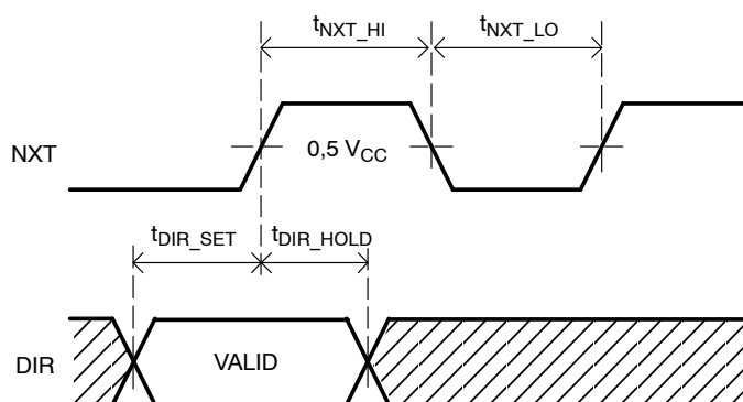
Figure 2. NXT-input Timing Diagram
