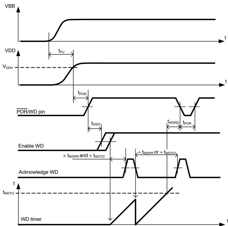
Figure 4. Watchdog Timing Diagram
