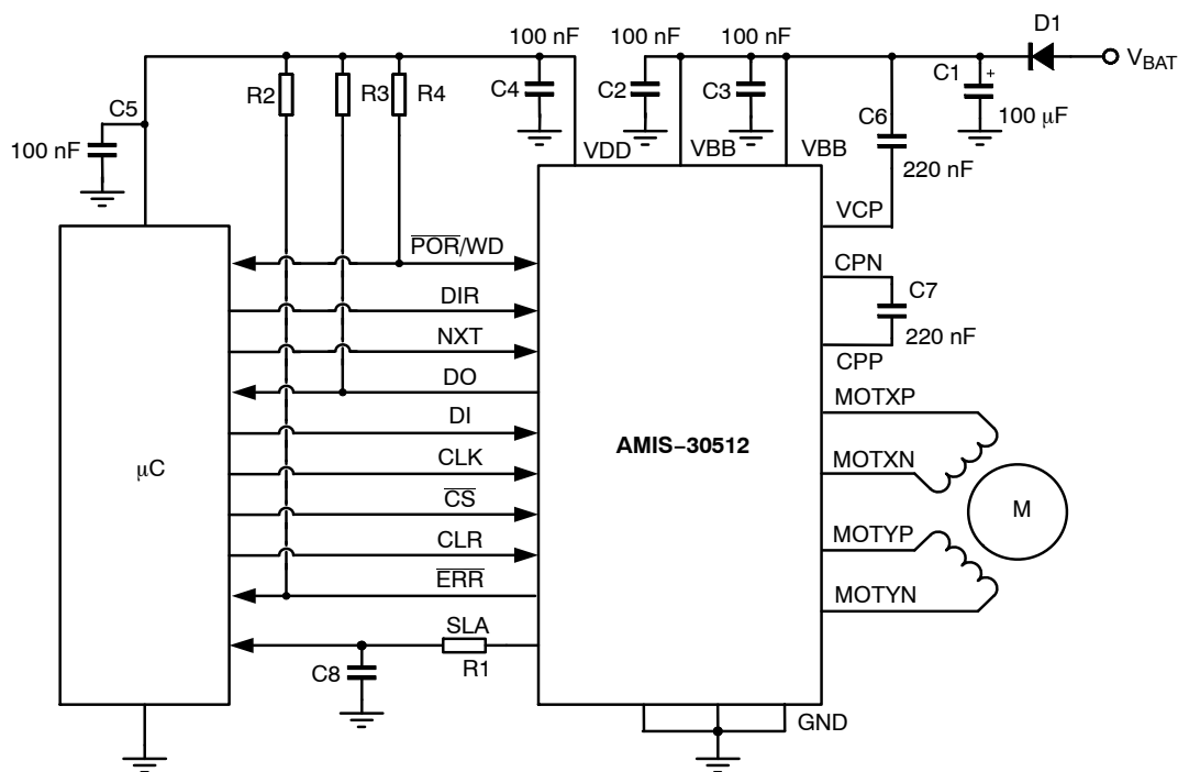
Figure 6. Typical Application Schematic
