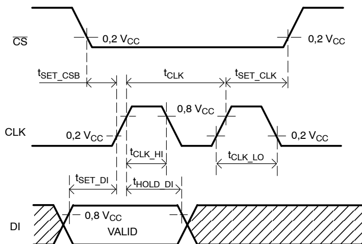
Figure 5. SPI Timing
