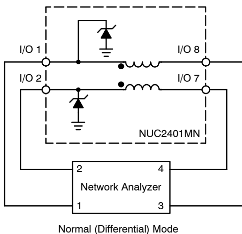
Figure 3. Normal (Differential) Mode Test Configuration
