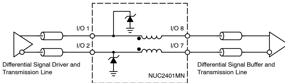
Figure 4. Application Circuit
