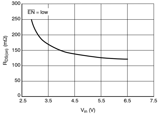
Figure 14. R_{DS(on)} vs. V_{in}
