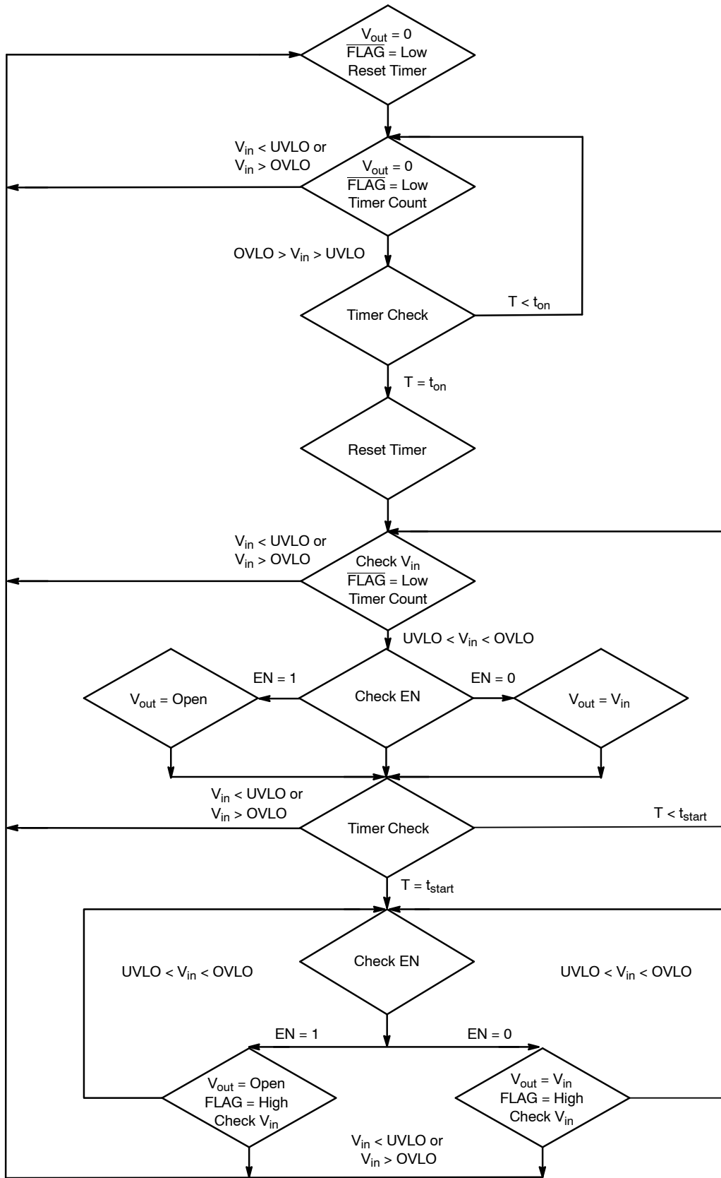
Figure 17. State Machine
