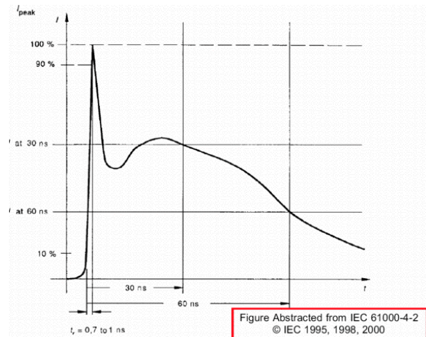
Figure 19. I_{peak} = f(t) /IEC61000-4-2
