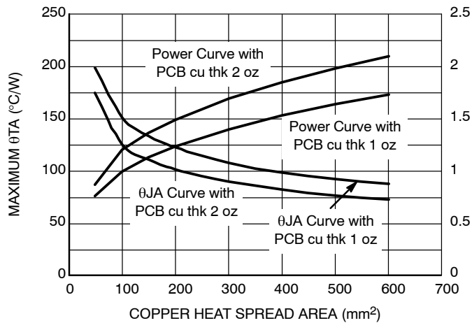
Figure 18. Copper heat Spread Area
