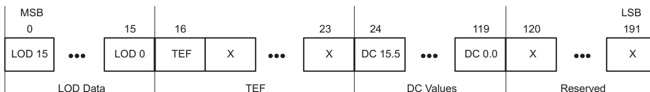
Figure 19. Status Information Data Packet Format
