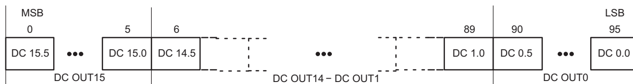
Figure 15. Dot Correction Data Packet Format
