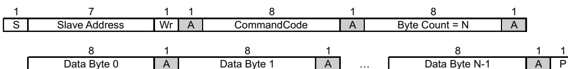
Figure 10. Block Write Protocol
