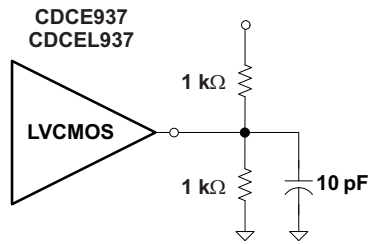
Figure 1. Test Load
