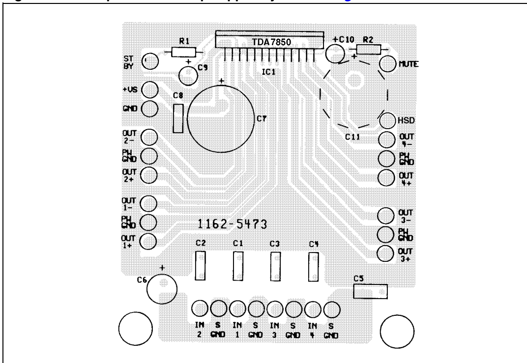
Figure 4. Components and top copper layer of the Figure 2 .
