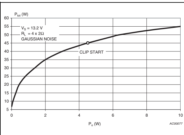
Figure 19. Power dissipation vs. output power ( R_L = 2\Omega , audio program simulation)
