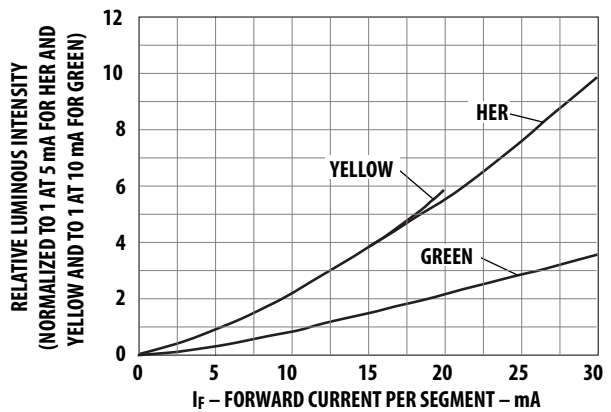
Figure 9. Relative luminous intensity vs. DC forward current.
