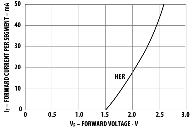
Figure 11. Forward current vs. forward voltage.
