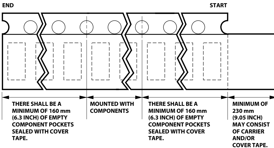
Figure 12. Tape leader and trailer dimensions.
