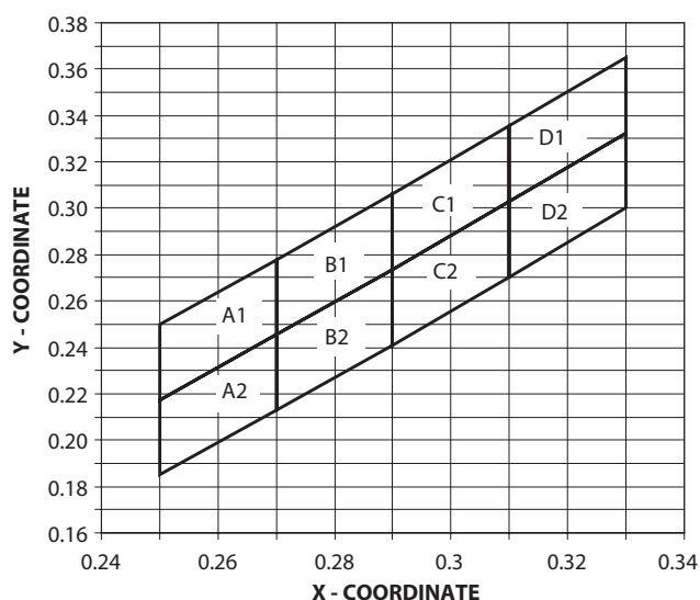
Figure 1. SMT White Color Bin Structure (CIE 1931 Chromaticity Diagram) [Tolerance = +/- 0.02]
