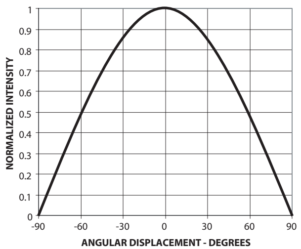
Figure 5. Radiation Pattern
