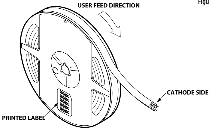
Figure 9. Reeling orientation.
