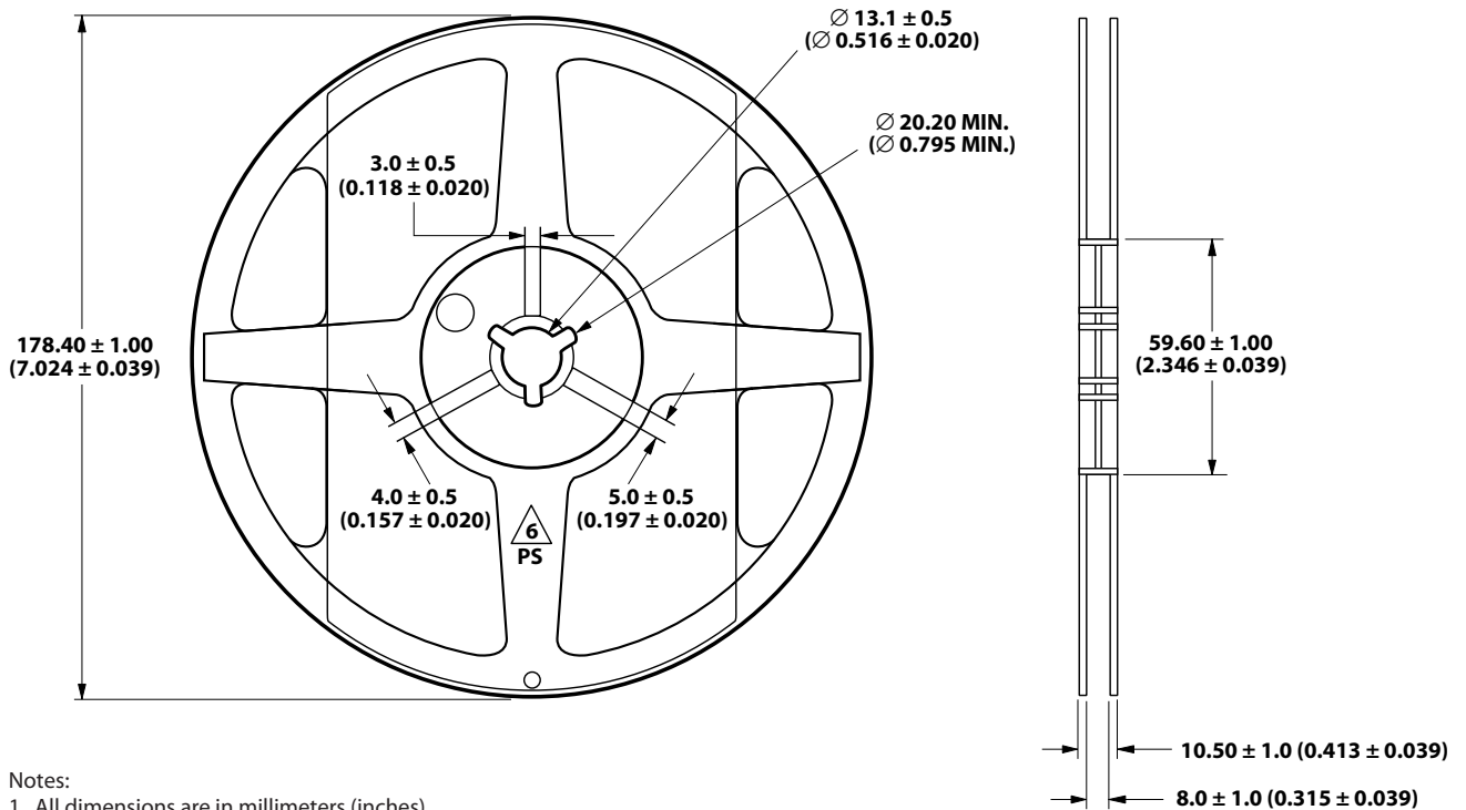
Figure 10. Reel dimensions.
