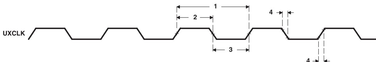
Figure 7-46 UXCLK Timing
