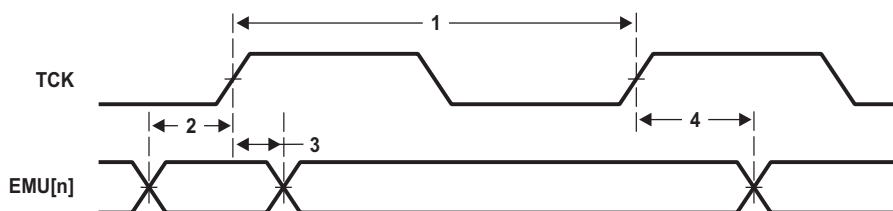
Figure 7-53 HS-RTDX Timing
