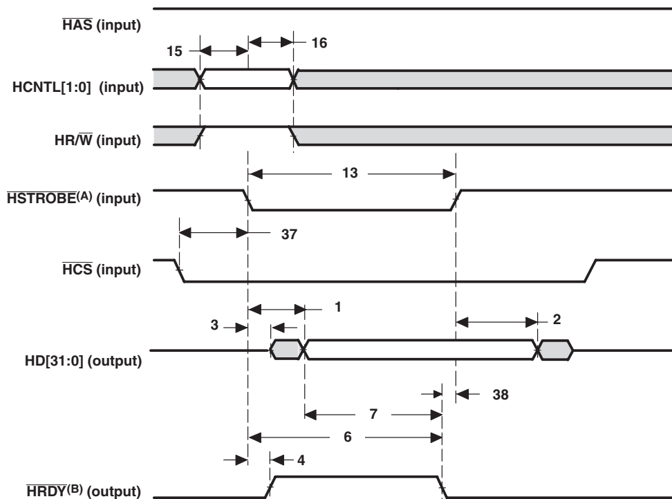
Figure 7-32 HPI32 Read Timing ( \overline{\text{H}}\overline{\text{A}}\overline{\text{S}} Not Used, Tied High)
