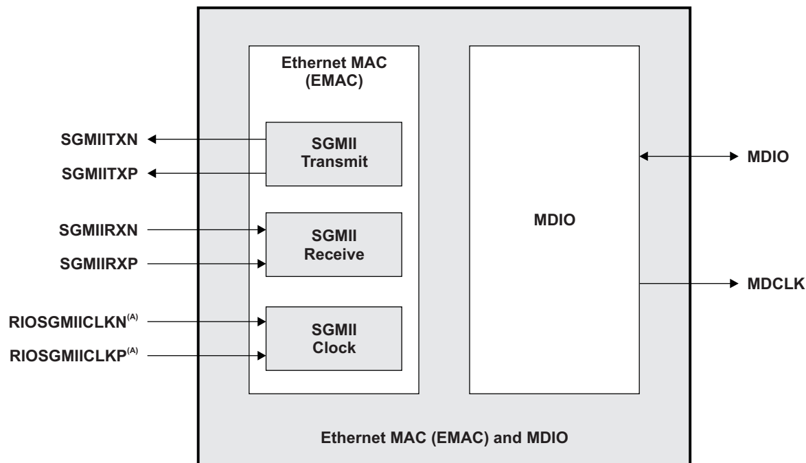
Figure 2-10 EMAC/MDIO (SGMII) Peripheral Signals
