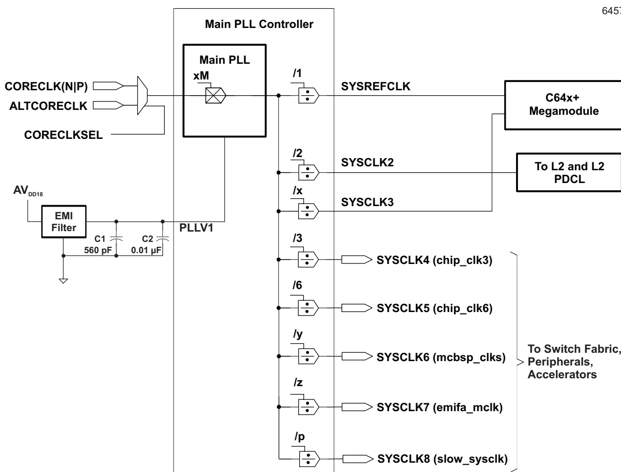
Figure 7-12 PLL1 and PLL1 Controller
