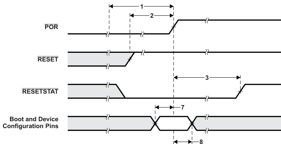
Figure 7-10 Warm Reset Timing — \overline{\text{RESETSTAT}} Relative to \overline{\text{RESET}}
