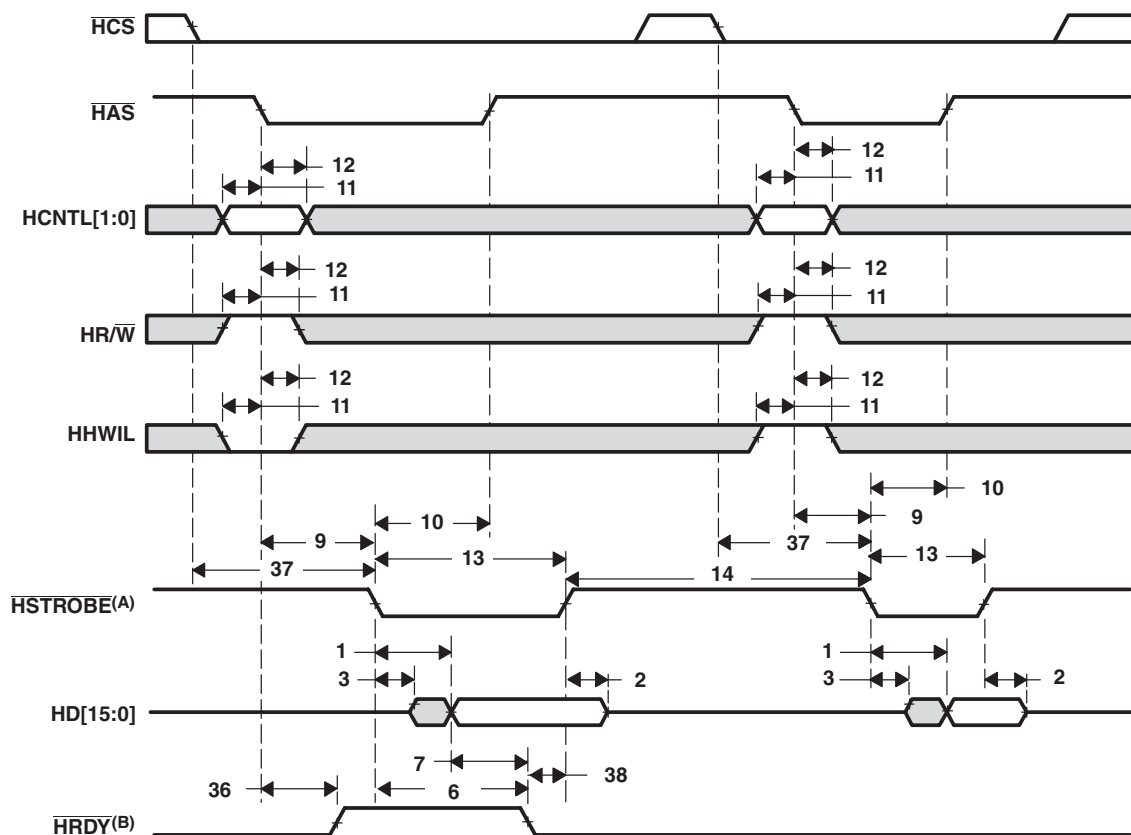
Figure 7-29 HPI16 Read Timing ( \overline{\text{HAS}} Used)
