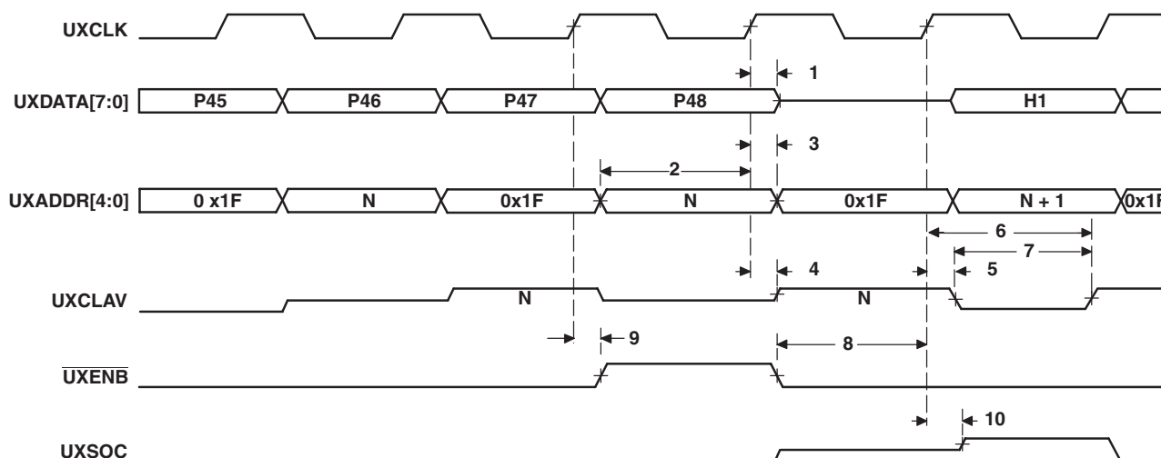
Figure 7-48 UTOPIA Slave Transmit Timing (A)
