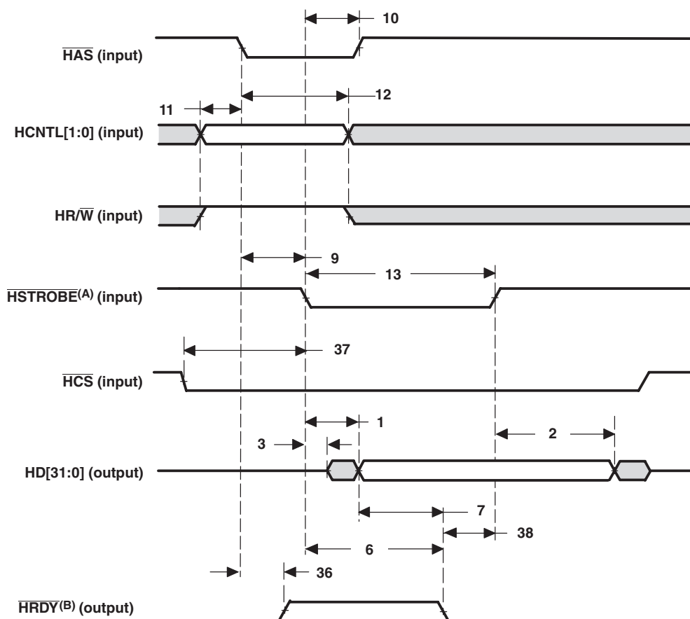
Figure 7-33 HPI32 Read Timing ( \overline{\text{HAS}} Used)
