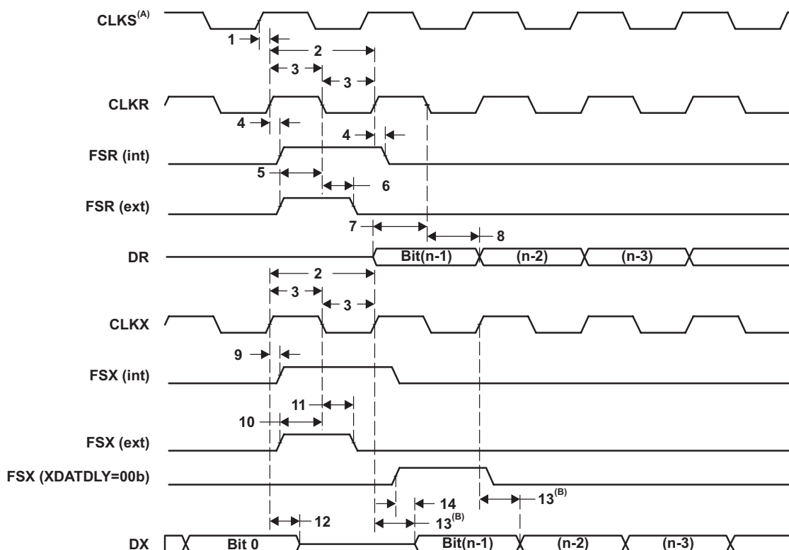
Figure 7-36 McBSP Timing
