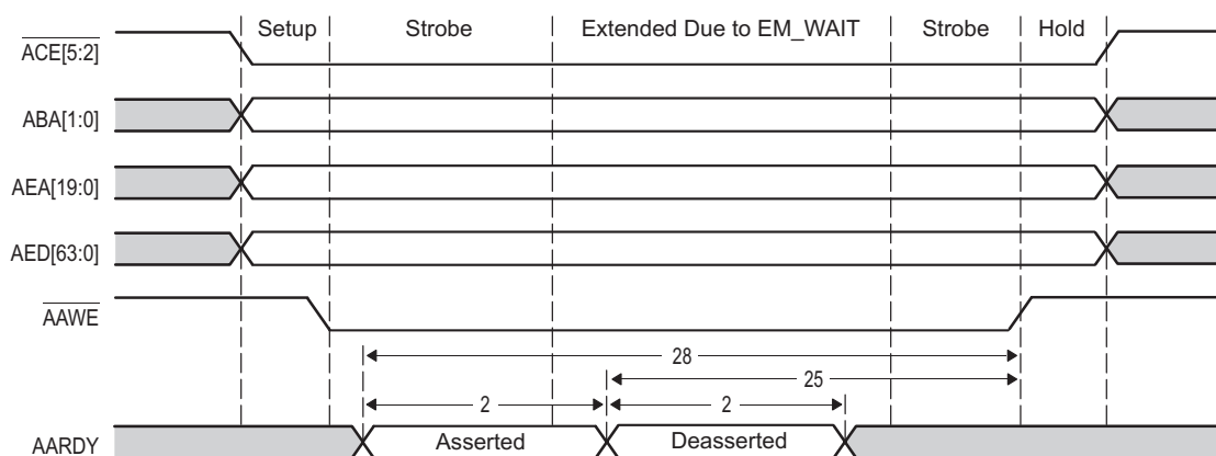
Figure 7-21 EMIFA EM_Wait Write Timing
