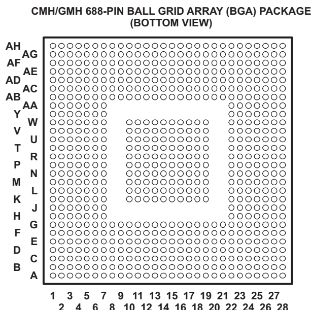
Figure 1-1 CMH/GMH 688-Pin Ball Grid Array (BGA) Package
