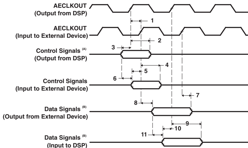
Figure 7-6 Board-Level Input/Output Timings
