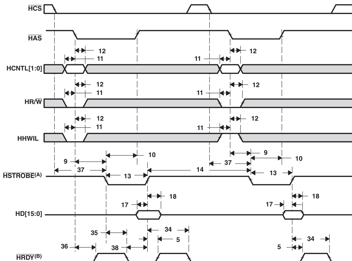
Figure 7-31 HPI16 Write Timing ( \overline{\text{HAS}} Used)
