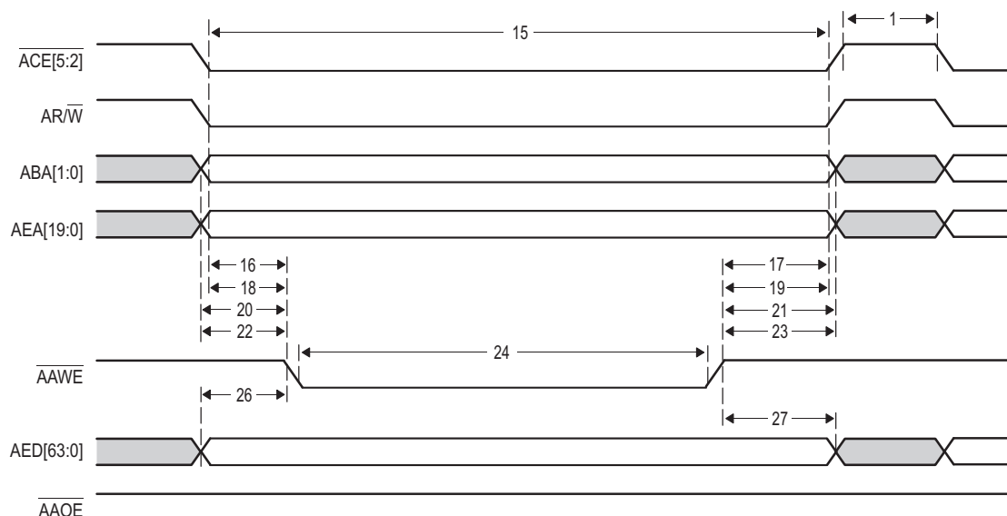
Figure 7-19 EMIFA Asynchronous Memory Write Timing
