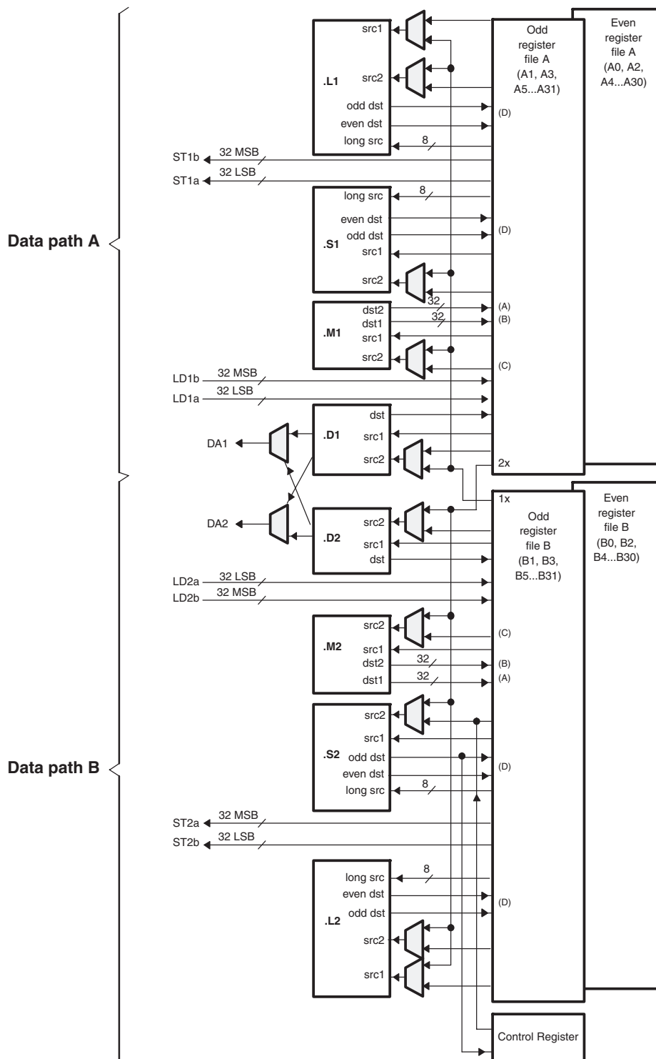
Figure 2-1 TMS320C64x+ CPU (DSP Core) Data Paths
