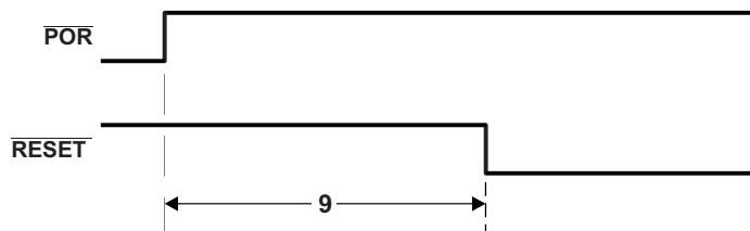
Figure 7-11 Warm Reset Timing — Setup Time Between \overline{\text{POR}} De-Asserted and \overline{\text{RESET}} Asserted
