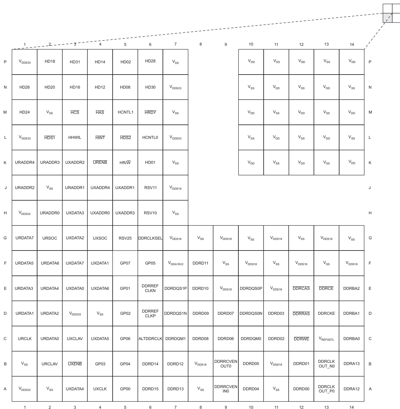
Figure 2-5 TMS320C6457 Pin Map (Bottom View) [Quadrant D]
