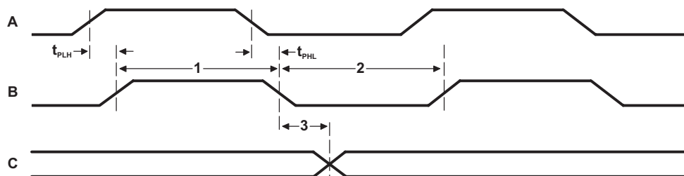
Figure 7-51 Trace Timing
