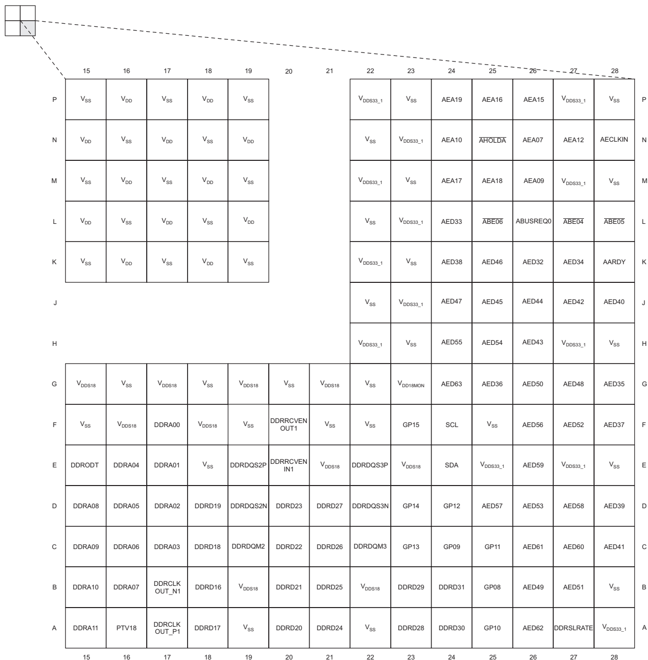
Figure 2-4 TMS320C6457 Pin Map (Bottom View) [Quadrant C]
