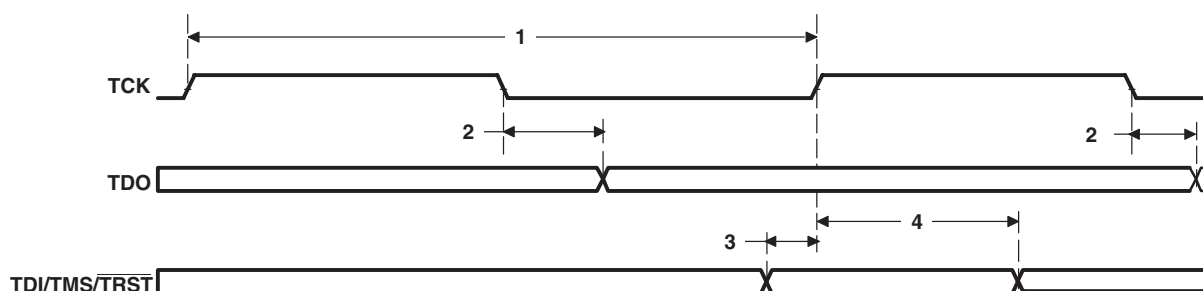
Figure 7-52 JTAG Test-Port Timing
