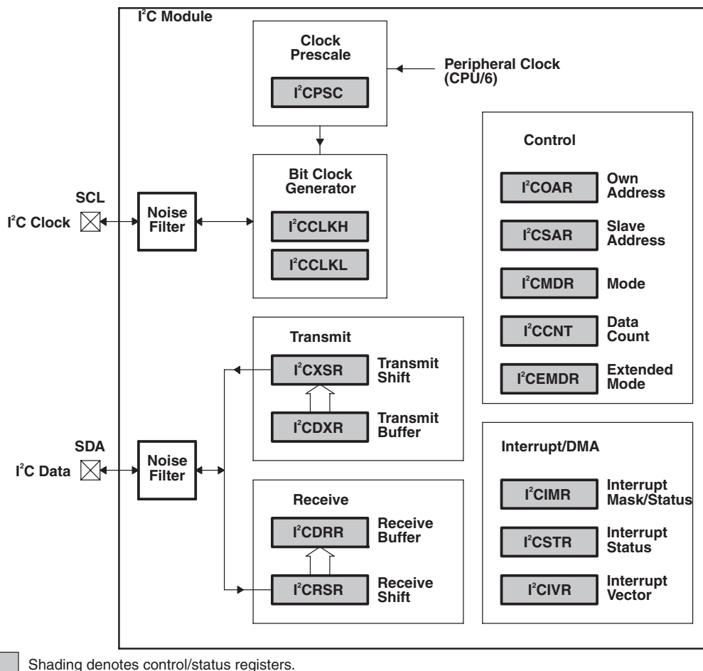
Figure 7-25 I 2 C Module Block Diagram
