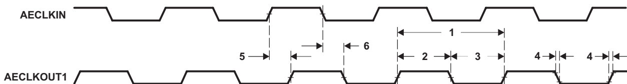
Figure 7-17 EMIFA AECLKOUT Timing
