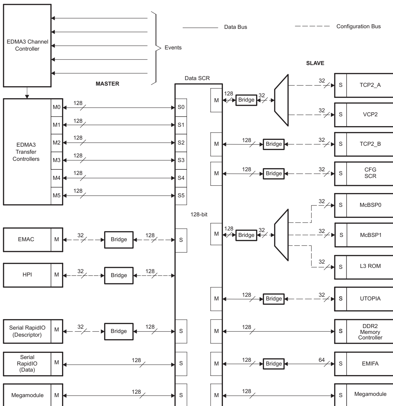
Figure 4-1 Data Switched Central Resource Block Diagram
