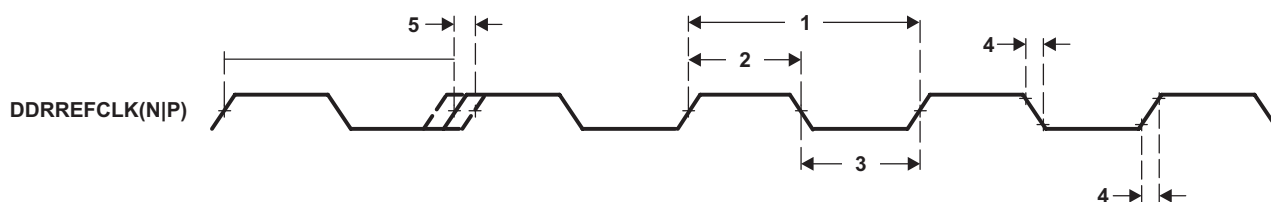
Figure 7-15 DDRREFCLK(N|P) Timing
