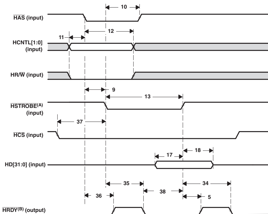
Figure 7-35 HPI32 Write Timing ( \overline{\text{HAS}} Used)
