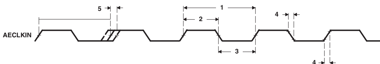
Figure 7-16 EMIFA AECLKIN Timing
