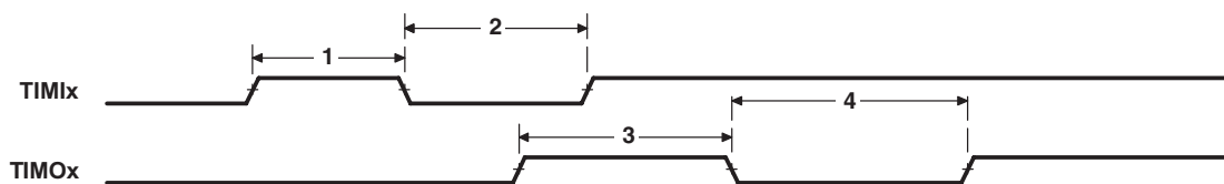
Figure 7-45 Timer Timing
