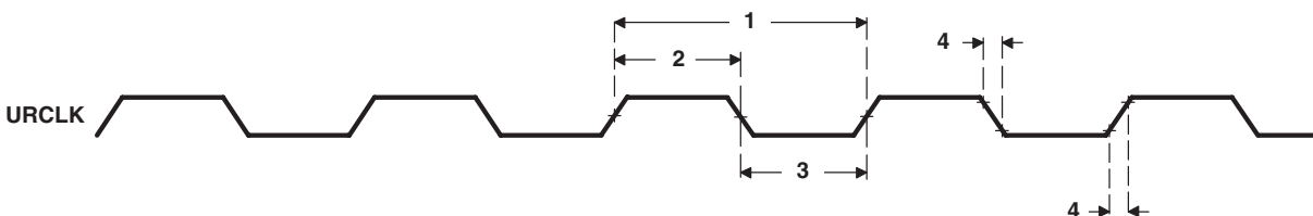
Figure 7-47 URCLK Timing
