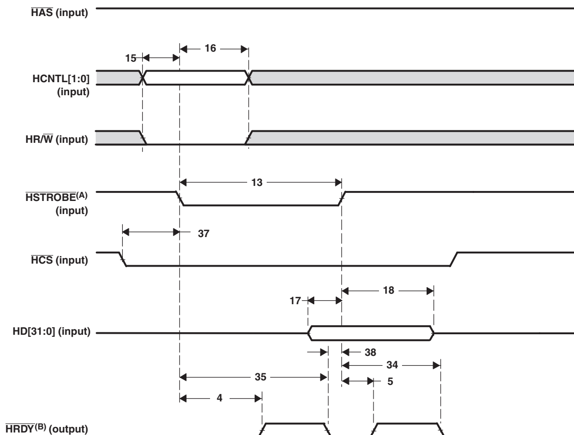
Figure 7-34 HPI32 Write Timing ( \overline{\text{HAS}} Not Used, Tied High)
