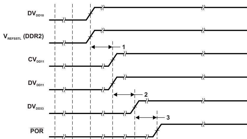
Figure 7-7 Power-Supply Sequence
