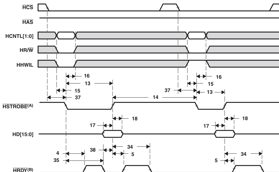
Figure 7-30 HPI16 Write Timing ( \overline{\text{HAS}} Not Used, Tied High)
