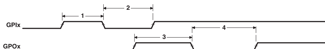
Figure 7-50 GPIO Timing
