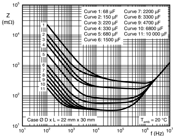
Fig. 11 - Typical impedance as a function of frequency
