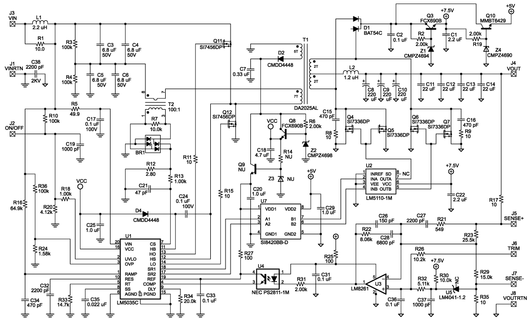
Figure 29. Evaluation Board Schematic
