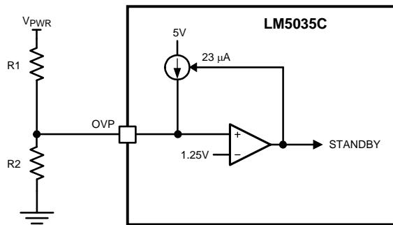
Figure 23. Basic Over-Voltage Protection
