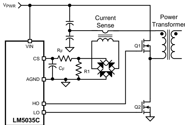
Figure 20. Current Sense Using Current Sense Transformer
