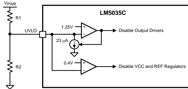
Figure 22. Basic UVLO Configuration
