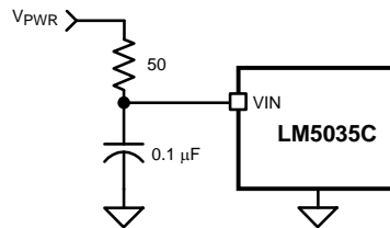
Figure 18. Input Transient Protection
