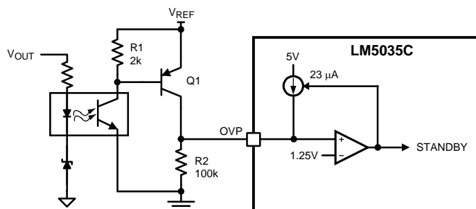
Figure 26. Latched Load Over-Voltage Protection
