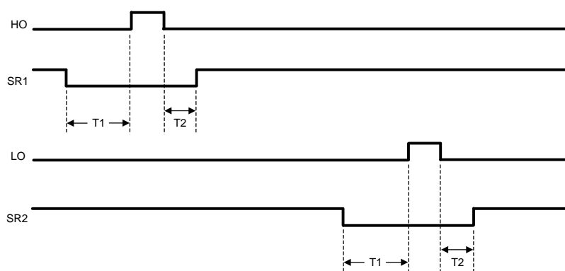
Figure 17. HO, LO, SR1 and SR2 Timing Diagram
