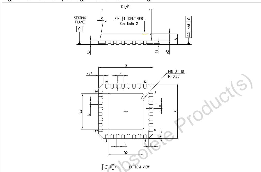
Figure 46. QFN32 package mechanical drawing
