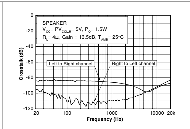
Figure 31. Crosstalk vs. frequency
