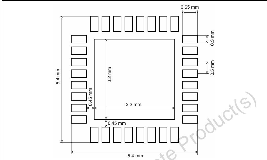
Figure 47. Footprint recommendation
