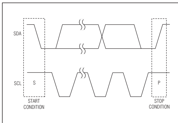
Figure 9. START and STOP Conditions
