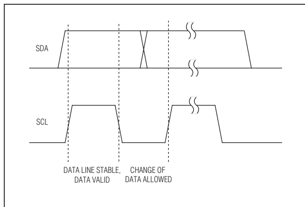
Figure 8. Bit Transfer
