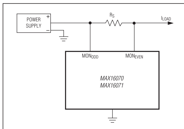
Figure 16. Current Monitoring Connection
