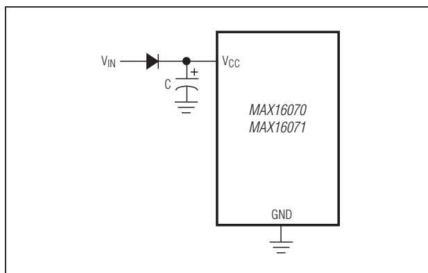
Figure 14. Power Circuit for Shutdown During Fault Conditions
