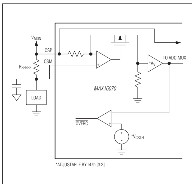
Figure 4. Current-Sense Amplifier
