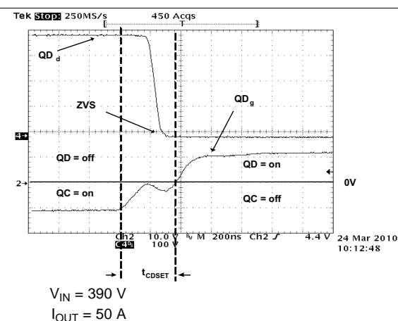
Figure 64. Full-Bridge Gate Drives and Switch Nodes ( QD_g QD_d )
