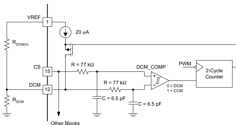
Figure 38. DCM Functional Block
