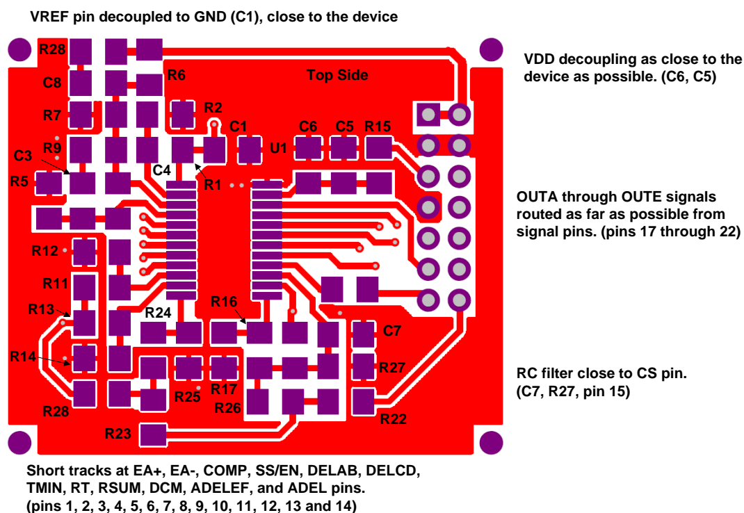
Figure 65. UCC28950 Layout Example (Top Side)
