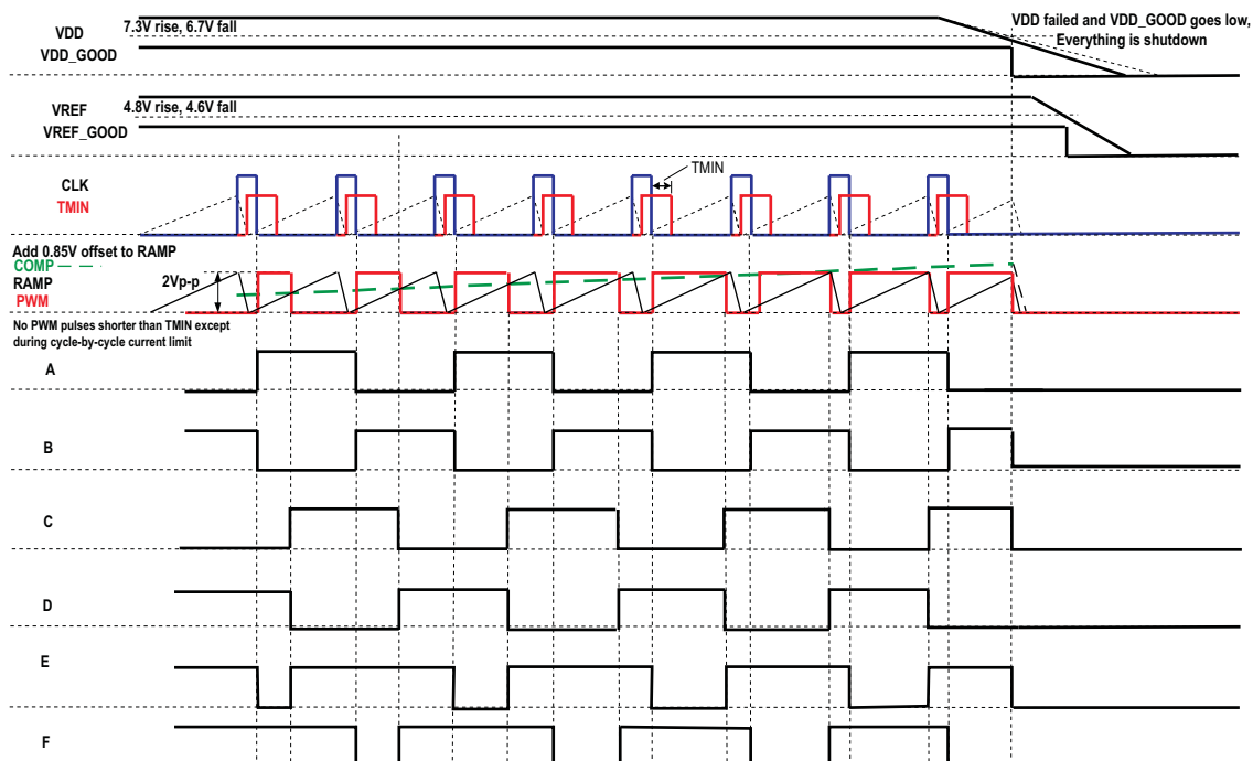
Figure 2. UCC28950 Steady State/Shutdown Timing Diagram
