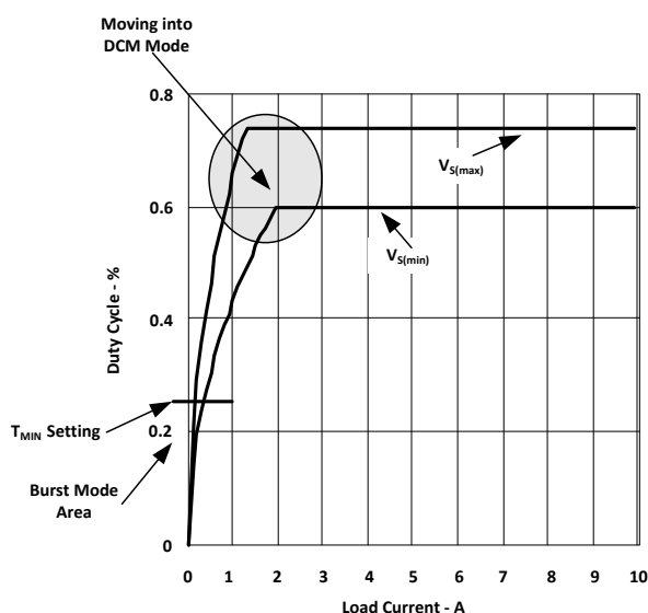
Figure 39. Duty Cycle Change Over Load Current Change
