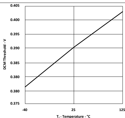
Figure 27. DCM Threshold vs Temperature
