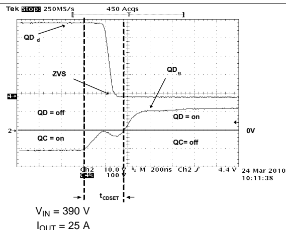
Figure 62. Full-Bridge Gate Drives and Switch Nodes ( QD_g QD_d )
