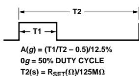
Figure 12. Typical Output Duty Cycle
