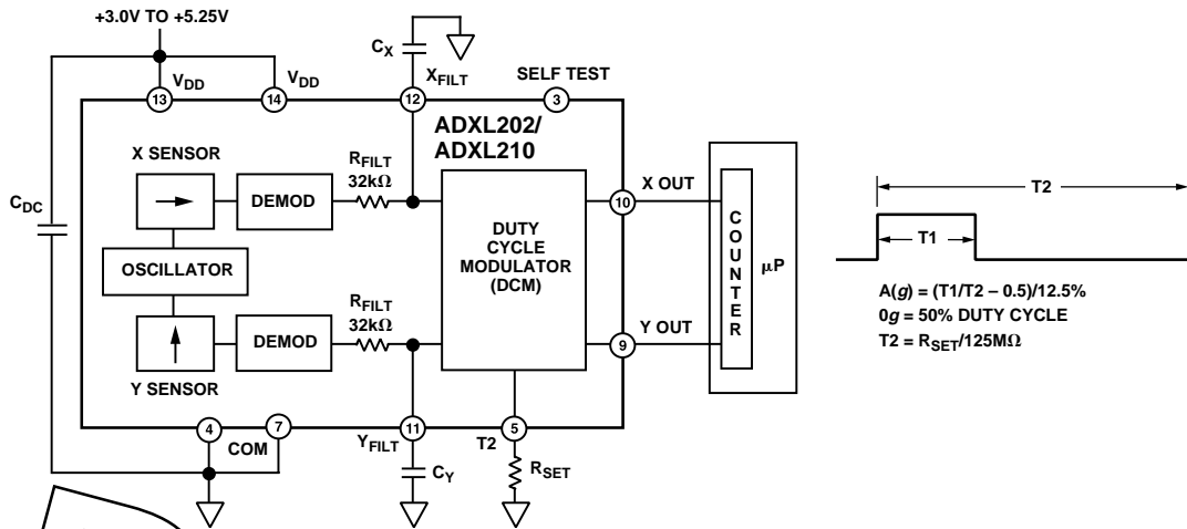
Figure 13. Block Diagram
