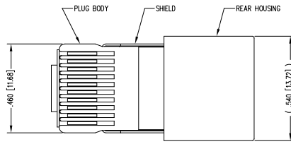
( SHOWN ASSEMBLED )
