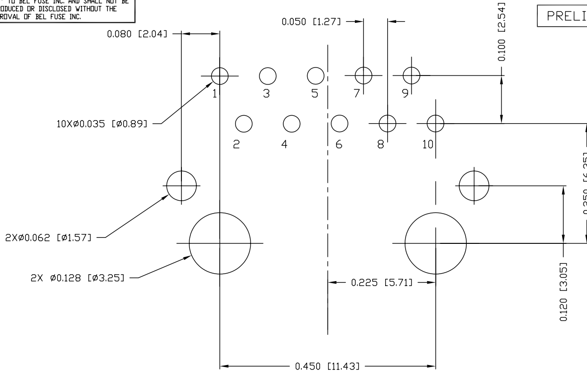
RECOMMENDED PCB FOOTPRINT COMPONENT SIDE VIEW
