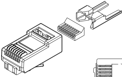
PLUG BODY
