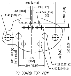
PC BOARD TOP VIEW
