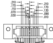
DIMENSIONS FOR KEY-26
