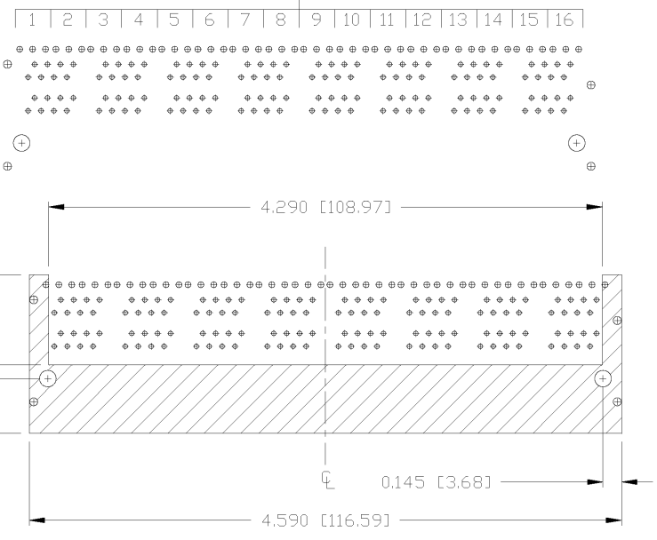
PORT ASSIGNMENT (COMPONENT SIDE VIEW)
