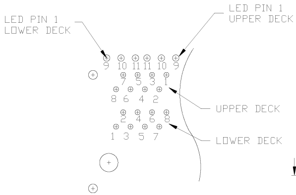
PIN-OUT INFORMATION (COMPONENT SIDE VIEW)
