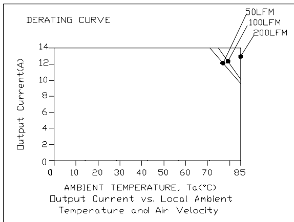
xRSB-40UV8x, Vin=48V
