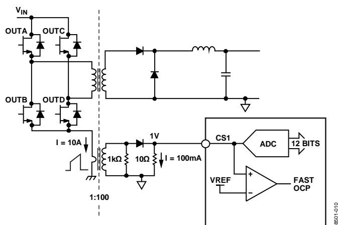
Figure 10. Current Sense 1 (CS1) Operation
