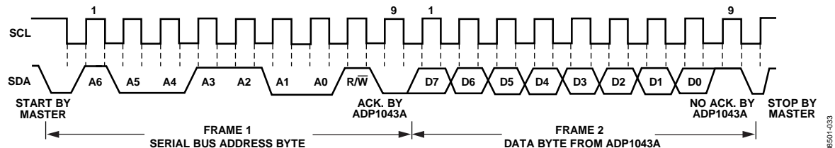
Figure 34. Reading Data from a Previously Selected Register
