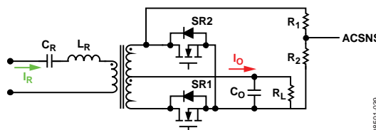
Figure 41. Resonant Synchronous Rectifier Control Circuit
