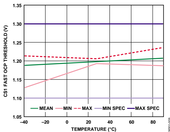
Figure 9. CS1 Fast OCP Threshold vs. Temperature
