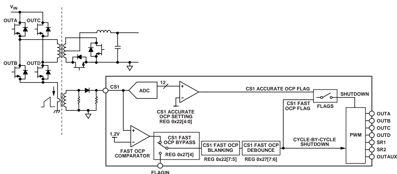
Figure 29. CS1 OCP Detailed Internal Schematic
