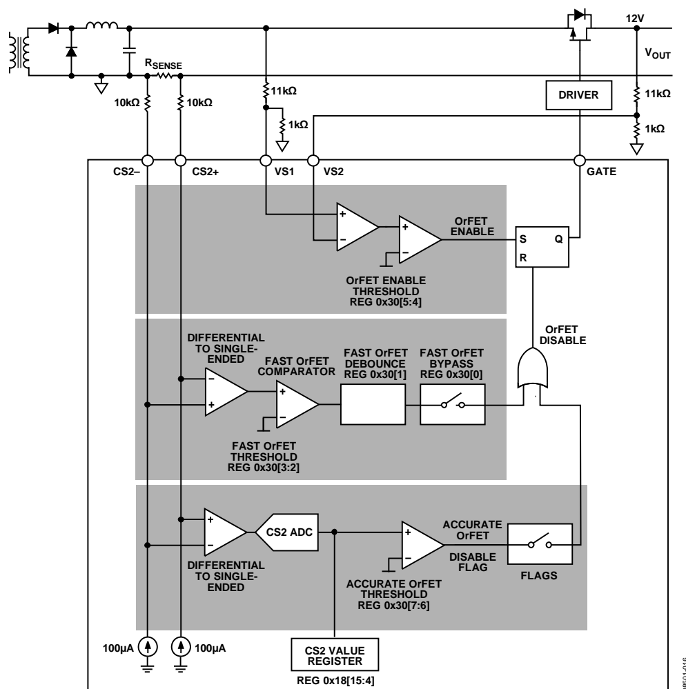
Figure 16. OrFET Control Circuit Internal Detailed Diagram
