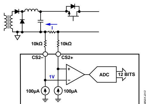
Figure 12. Low-Side Resistive Current Sense (Recommended)
