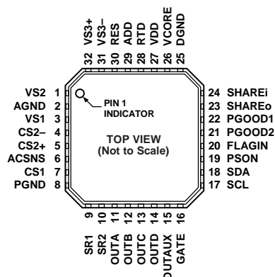
Figure 3. Pin Configuration
