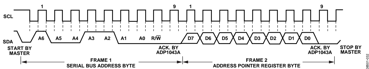
Figure 33. Writing to the Address Pointer Register Only
