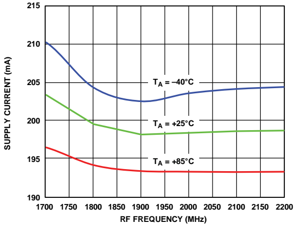
Figure 46. Supply Current vs. RF Frequency at 3.3 V
