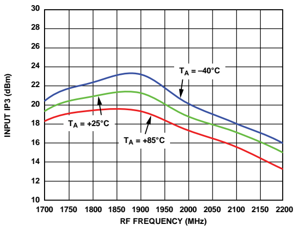
Figure 48. Input IP3 vs. RF Frequency at 3.3 V
