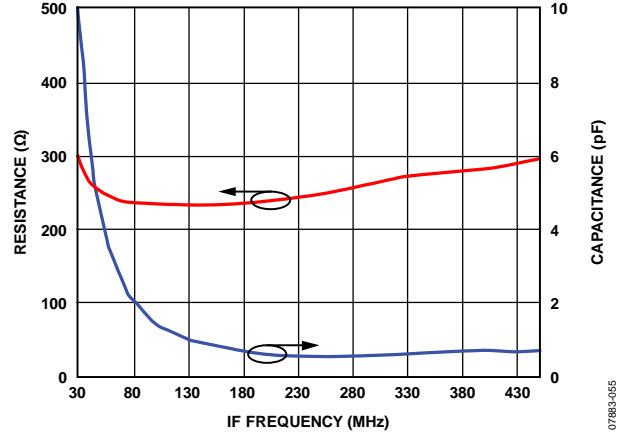
Figure 30. IF Output Impedance (R Parallel C Equivalent)
