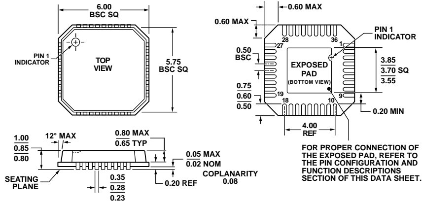
Figure 57. 36-Lead Lead Frame Chip Scale Package [LFCSP_VQ] 6mm x 6 mm Body, Very Thin Quad (CP-36-1) Dimensions shown in millimeters
