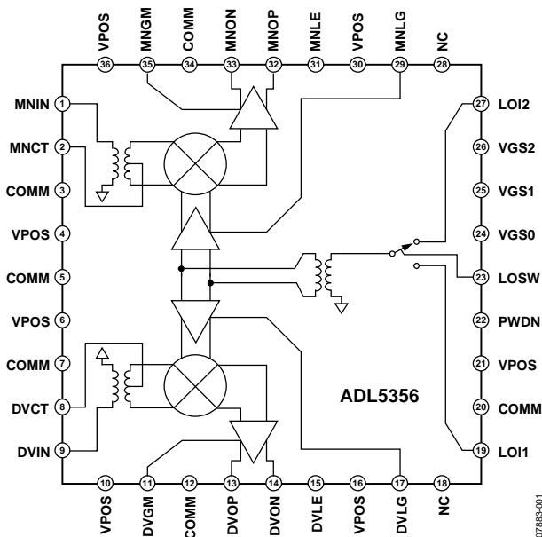
Figure 52. Simplified Schematic
